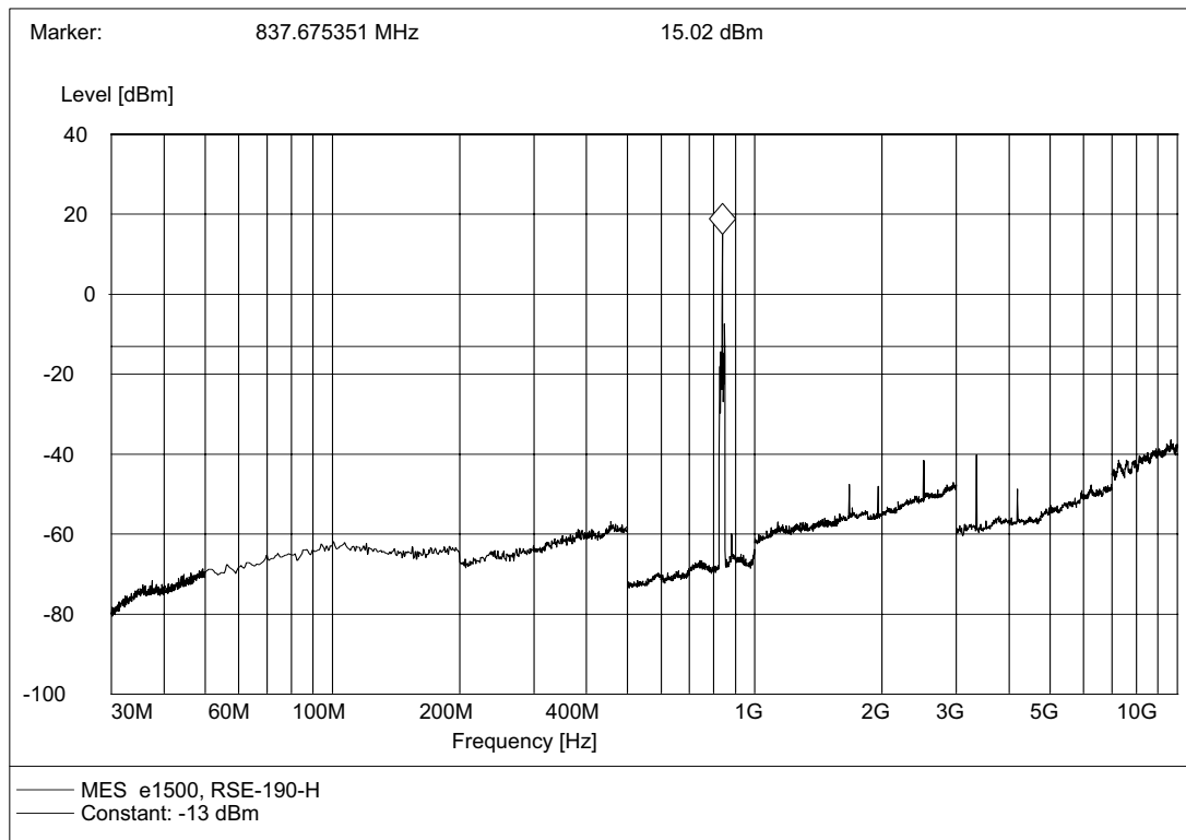
(Plot B.1: Channel = 190, Test Antenna Horizontal)
