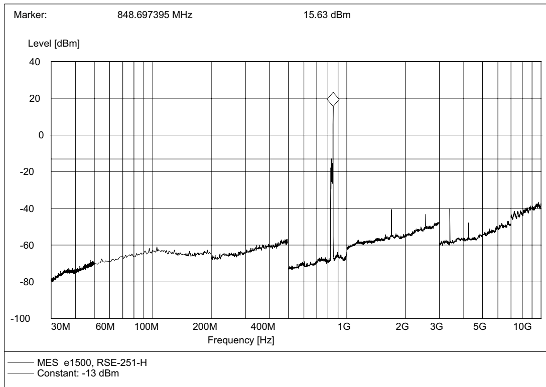
(Plot C.1: Channel = 251, Test Antenna Horizontal)
