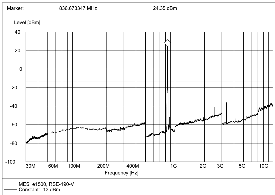
(Plot B.2: Channel = 190, Test Antenna Vertical)
