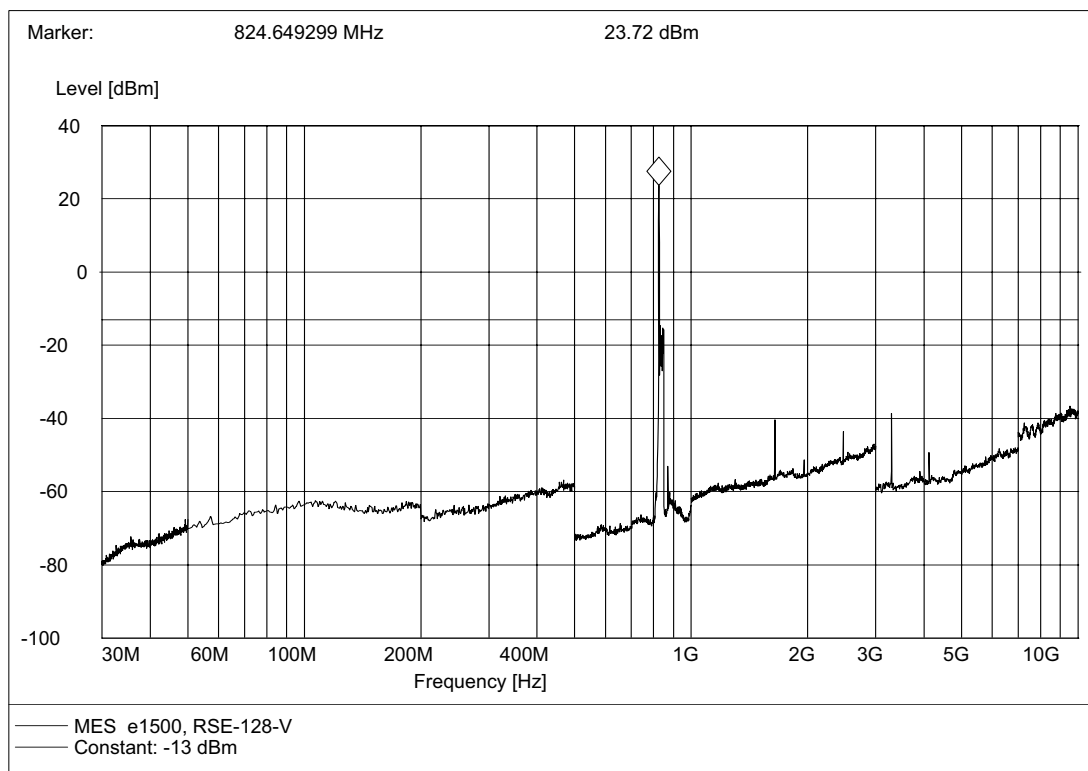
(Plot A.2: Channel = 128, Test Antenna Vertical)
