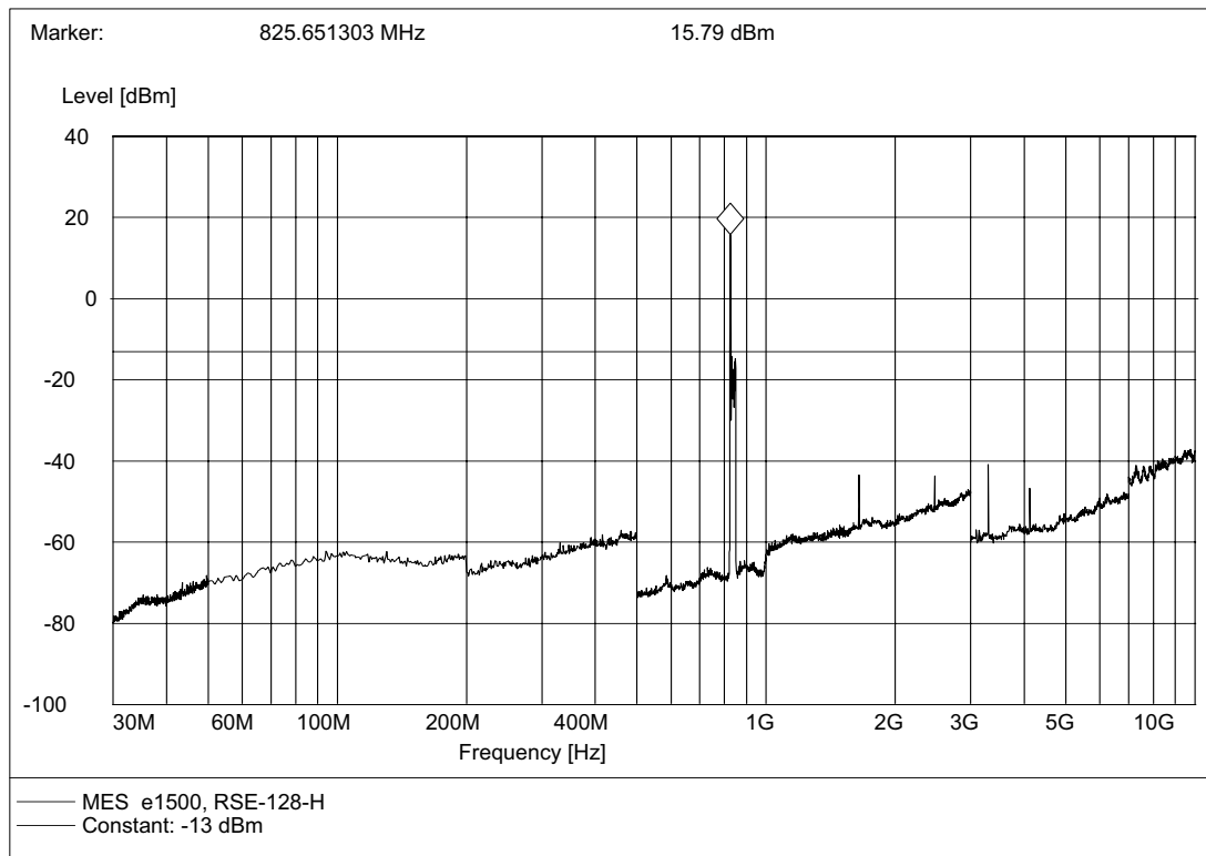
(Plot A.1: Channel = 128, Test Antenna Horizontal)
