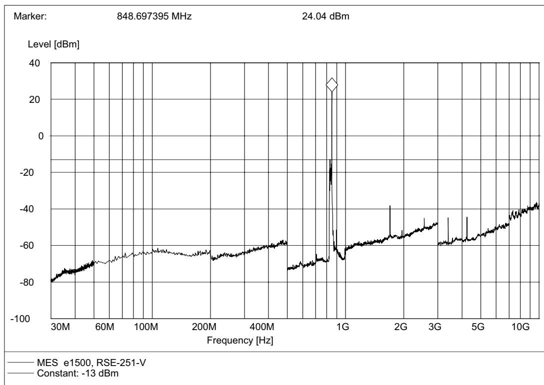
(Plot C.2: Channel = 251, Test Antenna Vertical)
