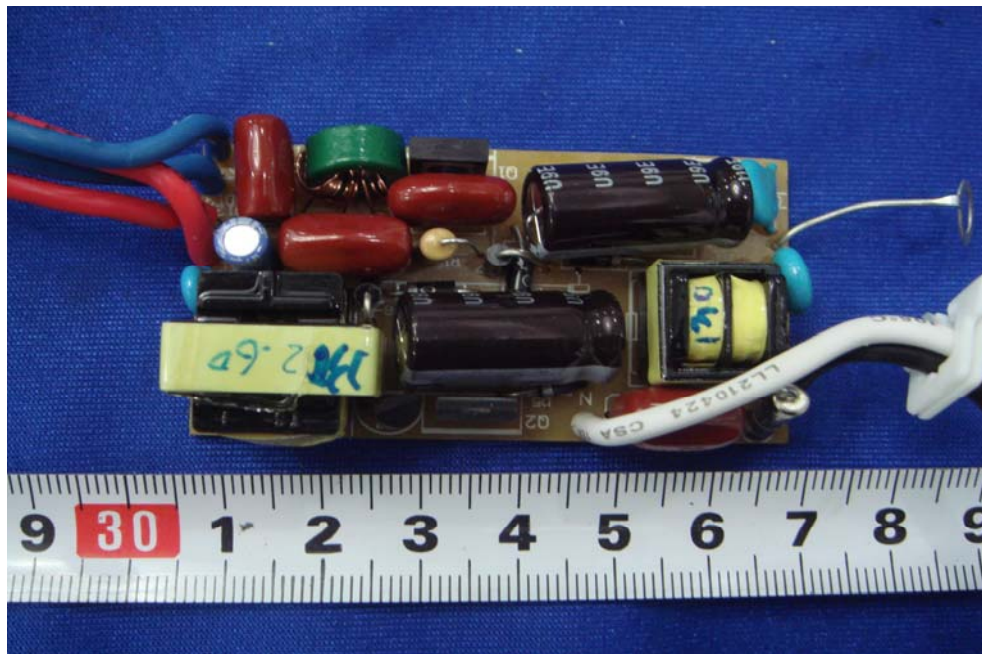
PCB-Front View for EBU130MA (30W)
