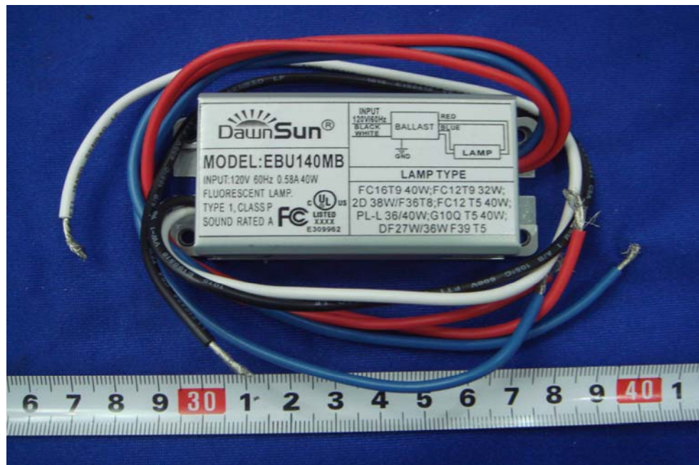
EUT-Front View for EBU140MB (40W)
