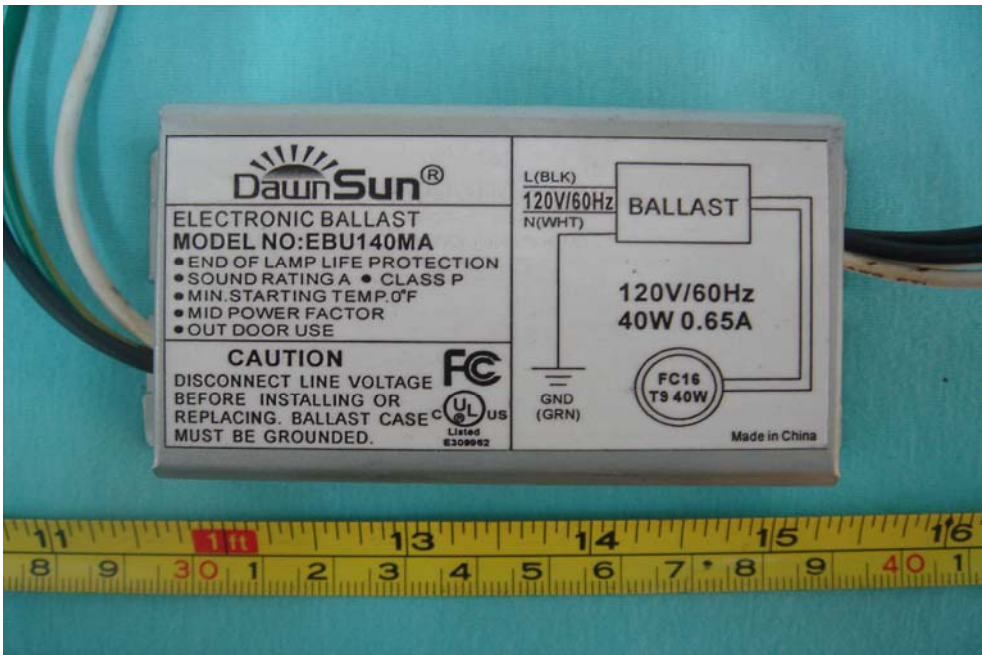
EUT-Back View for EBU140MA (40W)
