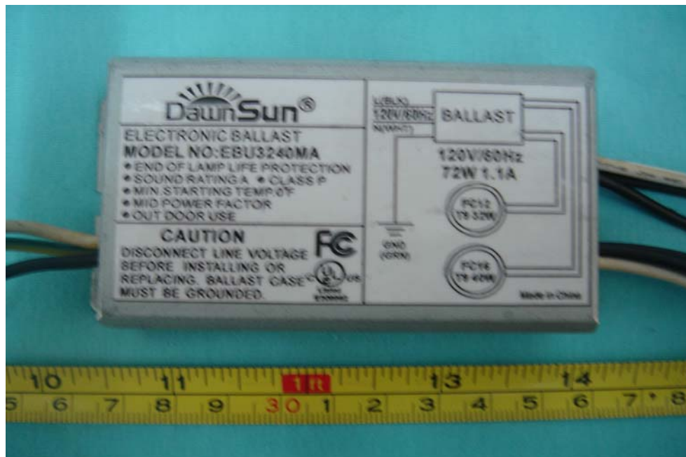
EUT-Front View for EBU3240MA (72W)
