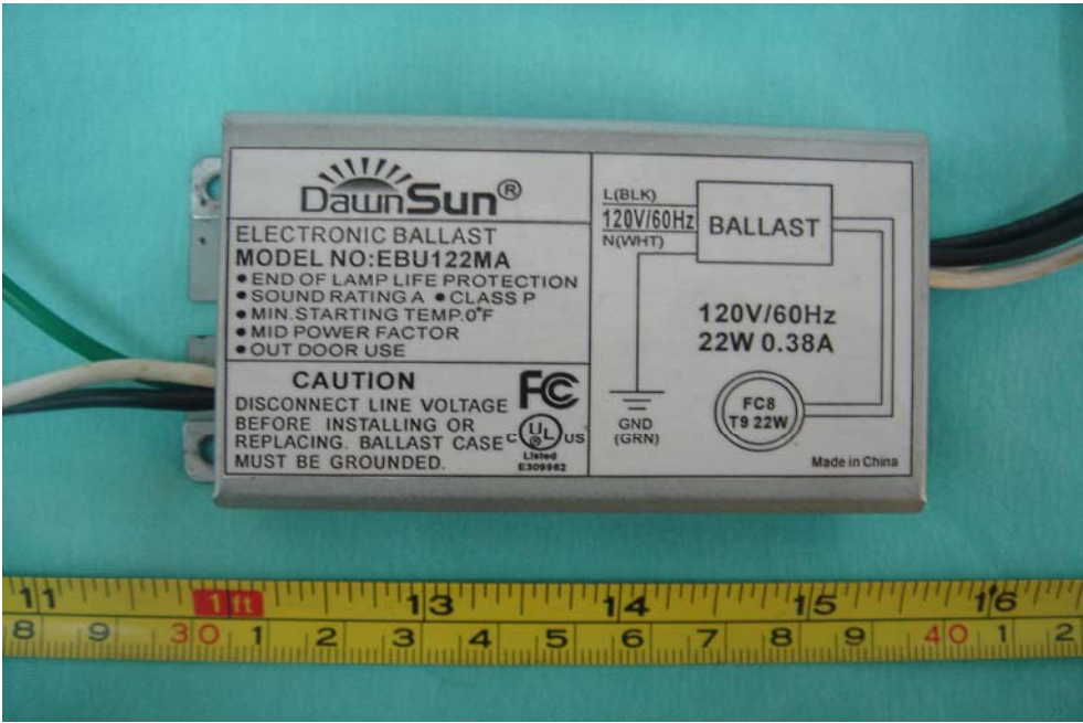
EUT-Back View for EBU122MA (22W)
