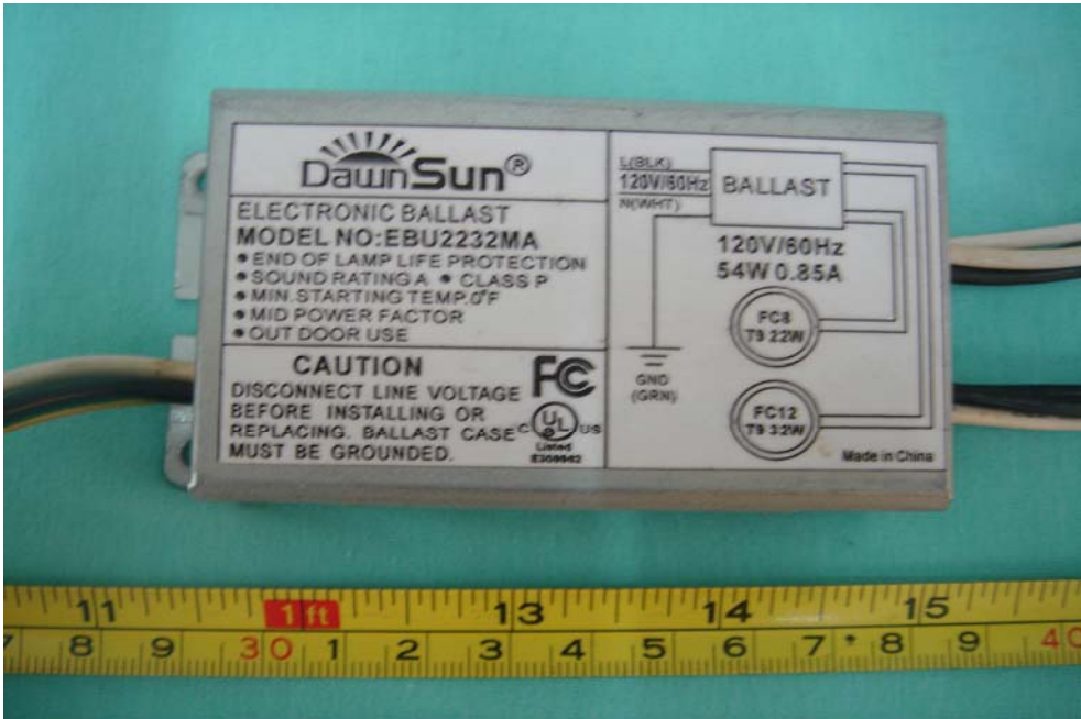
EUT-Back View for EBU2232MA (54W)
