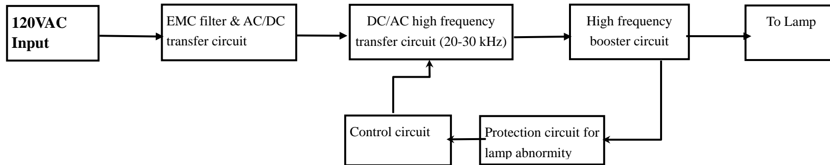
Basic block diagram of EBU***M* series electronic ballast
