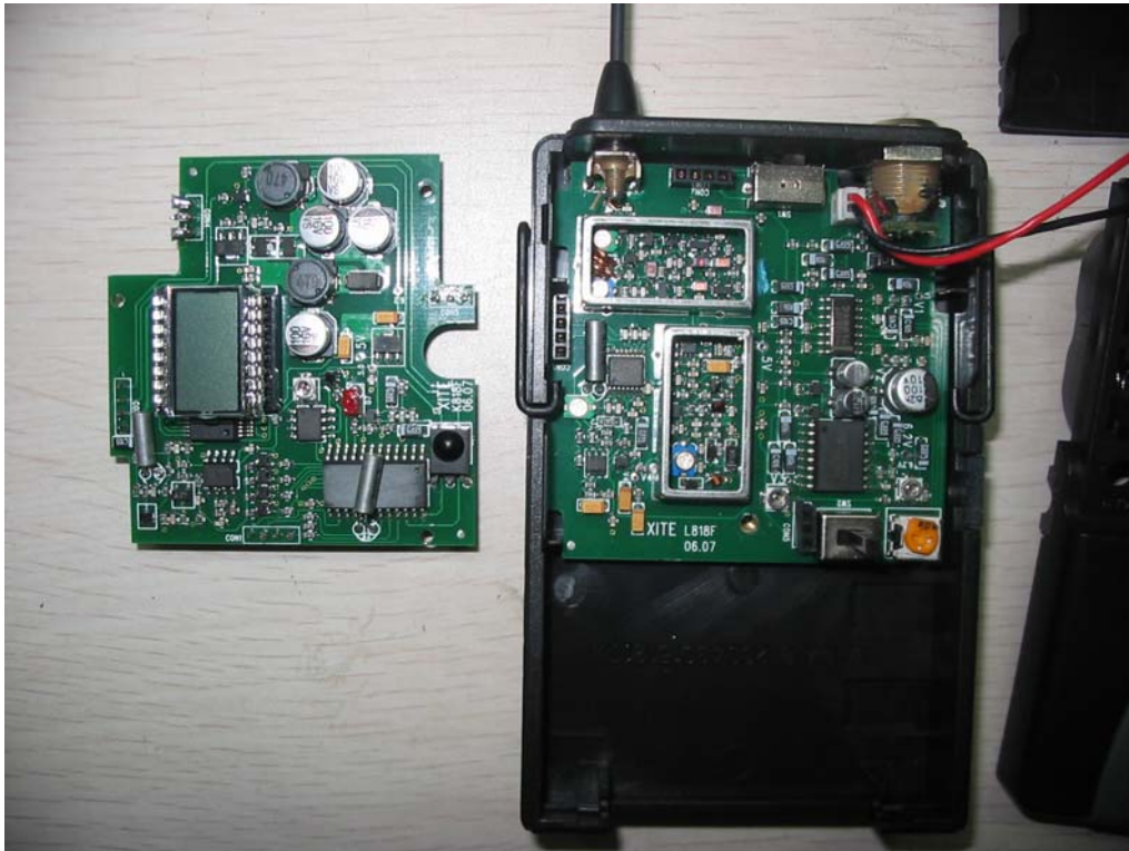
Internal View of Body worn Microphone-3
