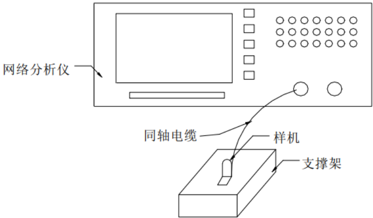
Figure 1 Wiring diagram of assembly test for microwave chamber system
