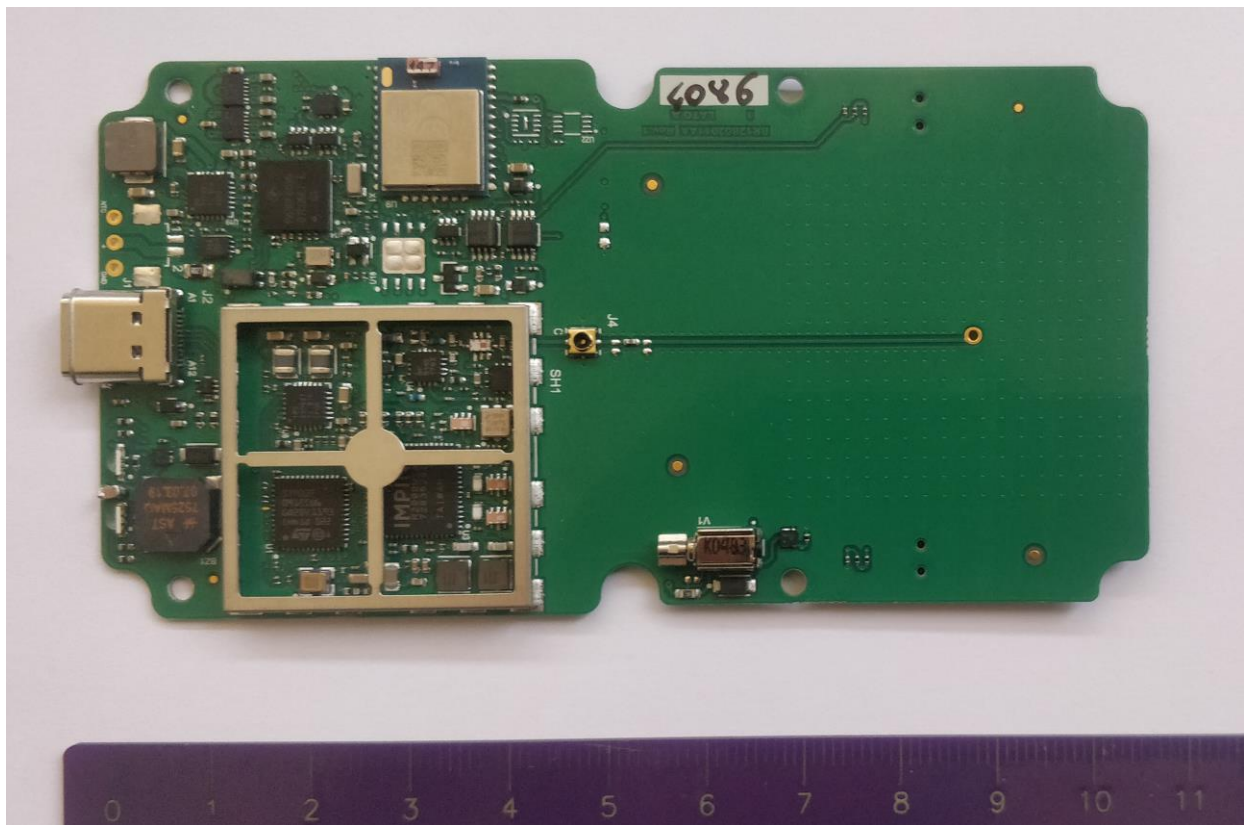
Figure 1: PCB top side
