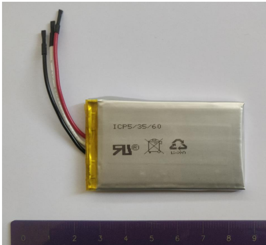
Figure 8: Battery pack (bottom side)
