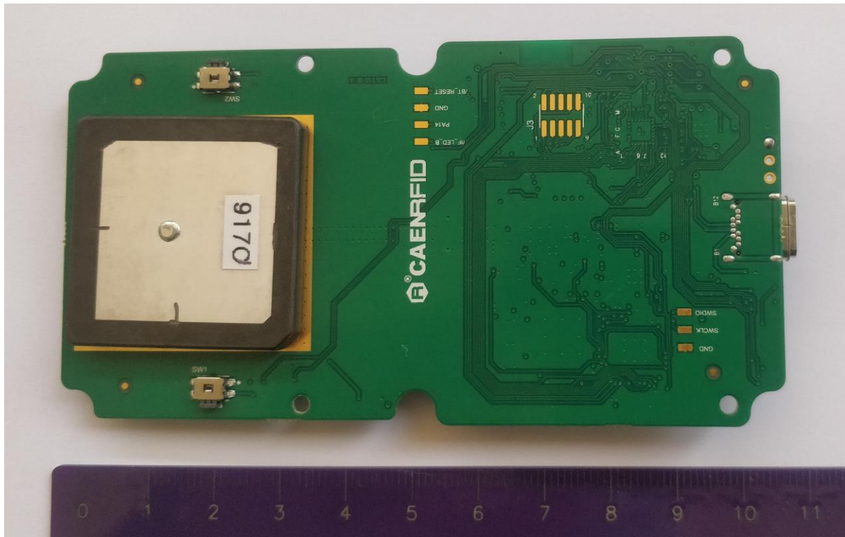
Figure 4: PCB bottom side with RFID antenna installed
