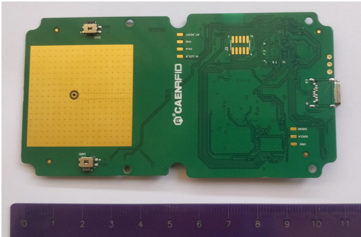
Figure 2: PCB bottom side
