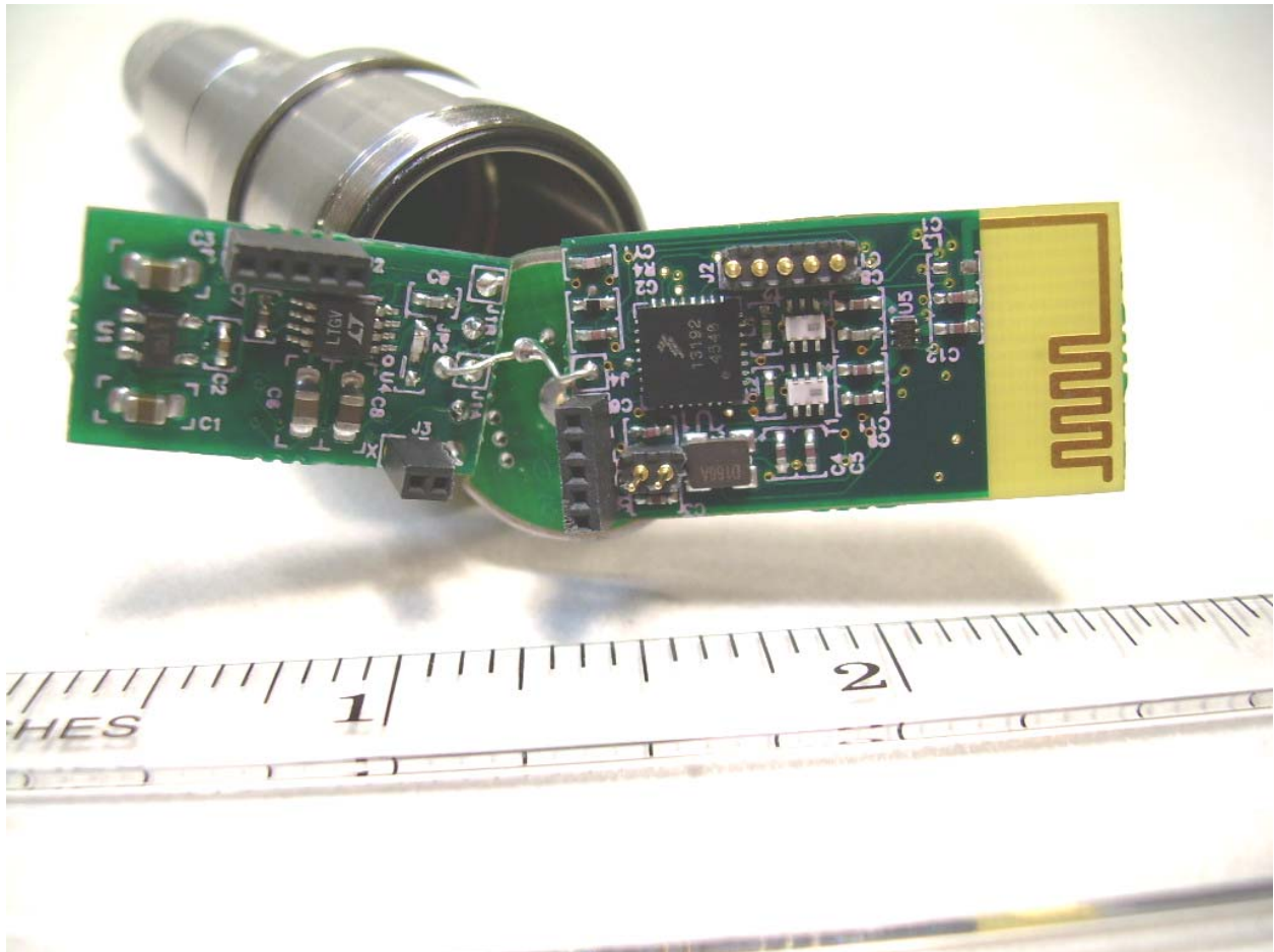
Photograph 15 - Inside View of the PCBs
