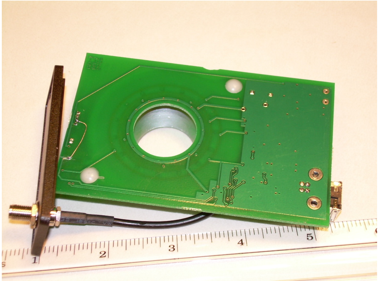
Photograph 9 - View of the Trace Side of the MPRF-H PCB
