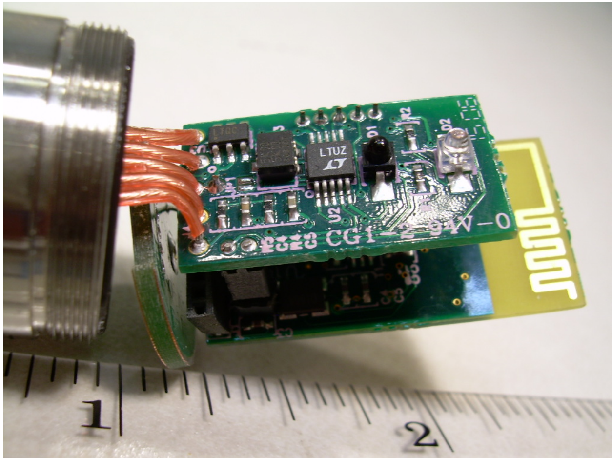
Photograph 14 - View of the Top Side of the Serial PCB
