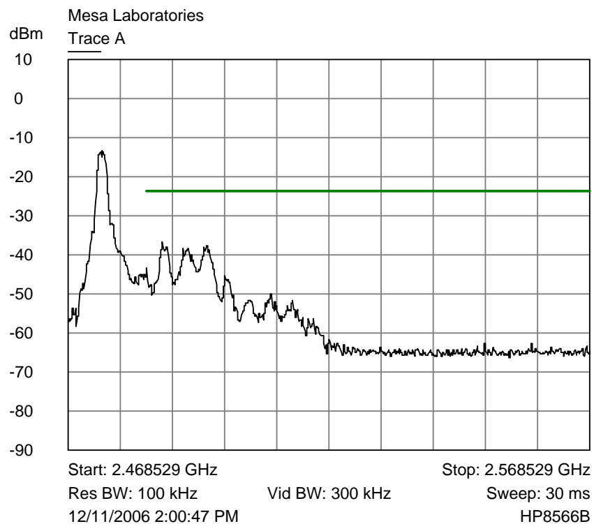
Trace A Ch 14 band edge plot
