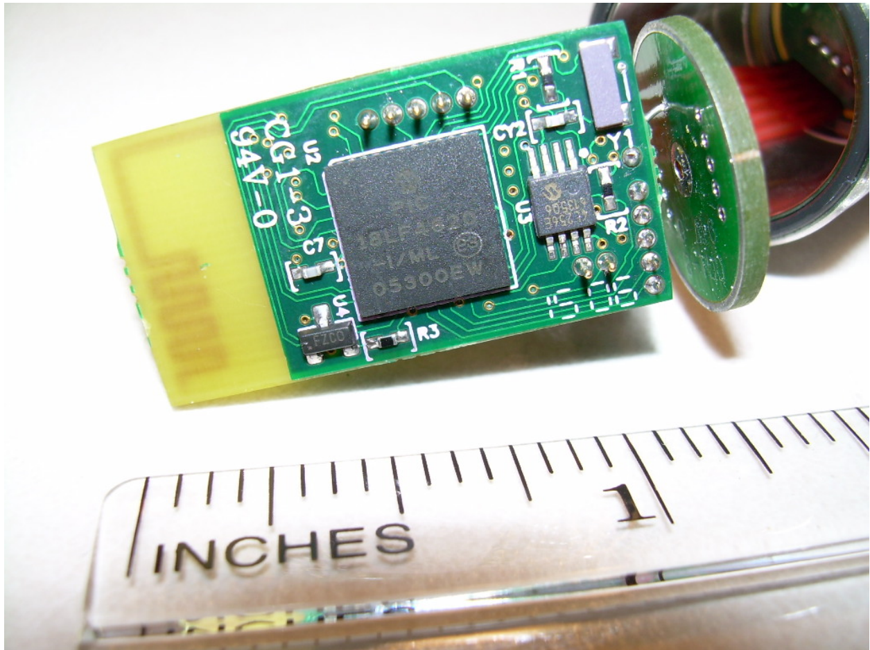
Photograph 13 - View of the Top Side of the Transceiver PCB
