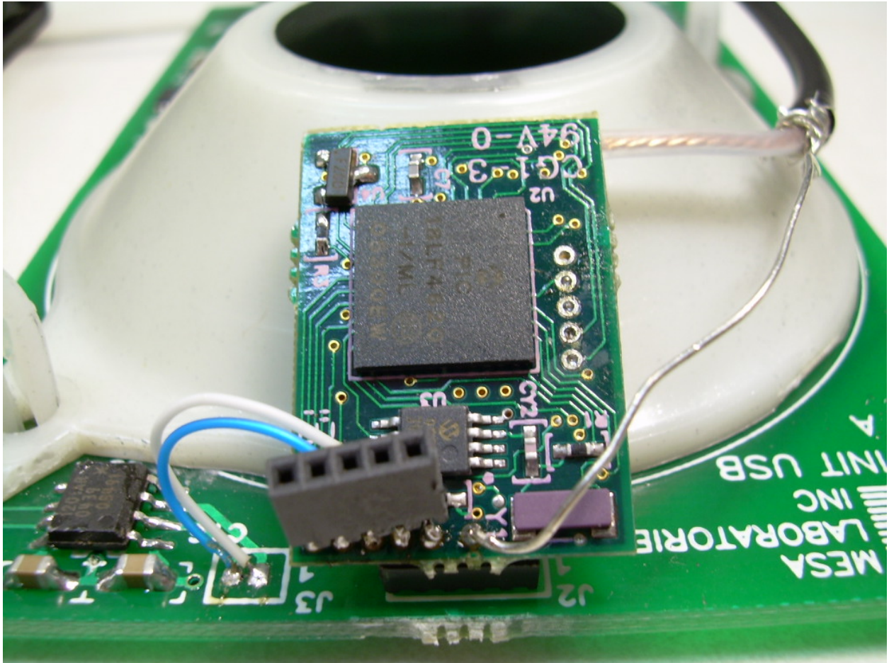
Photograph 10 - View of the Transceiver PCB
