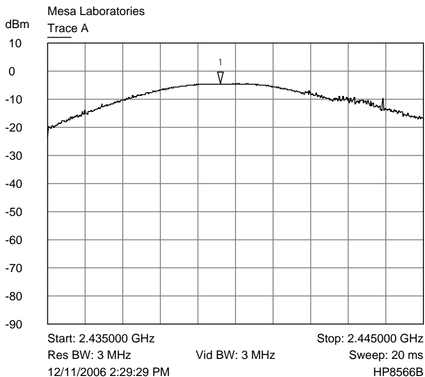
Trace A Ch 7 output power plot
