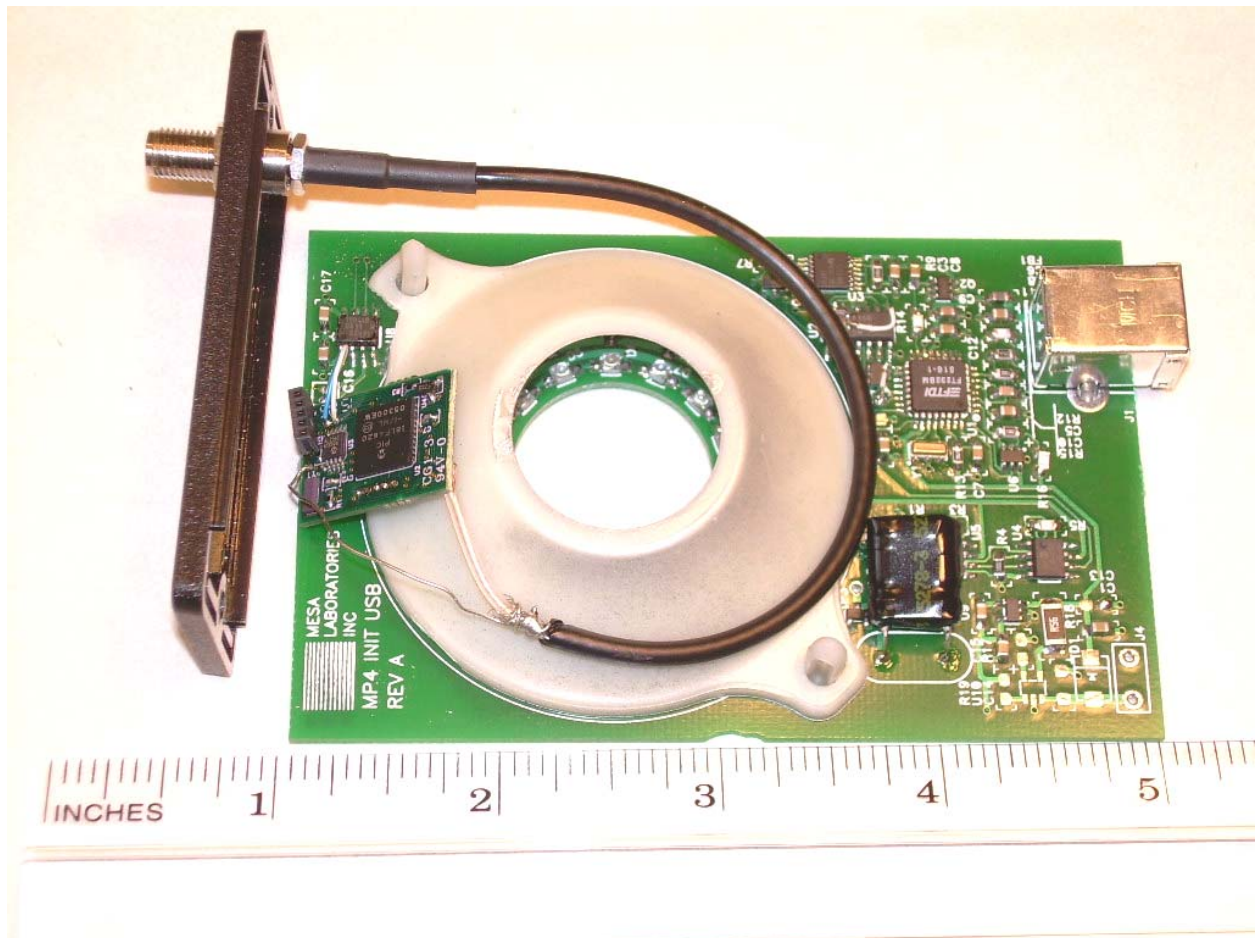
Photograph 7 - View of the Component Side of the MPRF-H PCB
