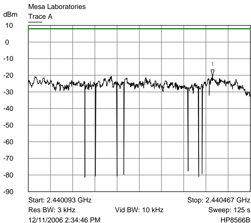
Trace A Ch 7 3 kHz power spectral density plot
