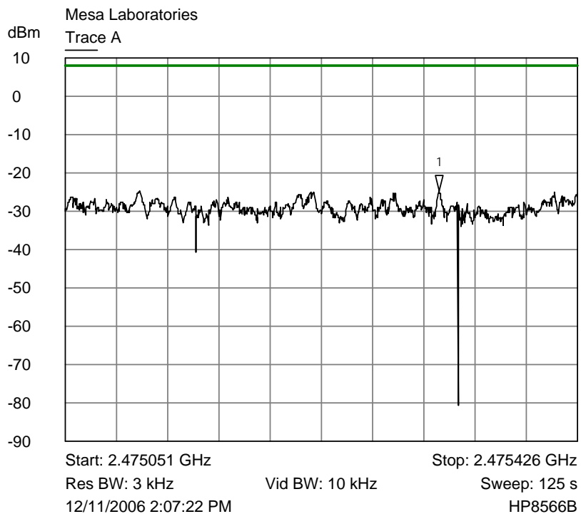
Trace A Ch 14 3 kHz power spectral density plot
