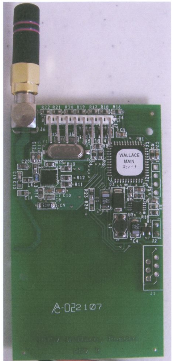
PCB back
