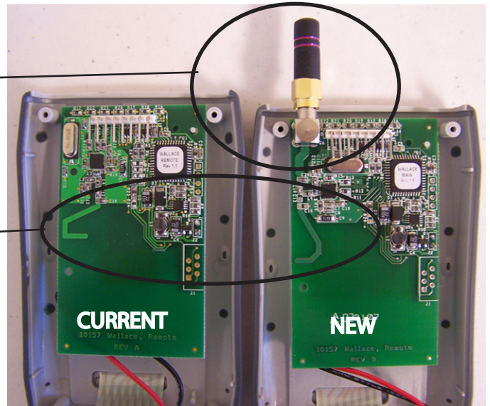
PCB back shown in enclosure
