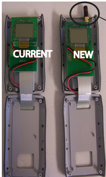
PCB front shown in enclosure
