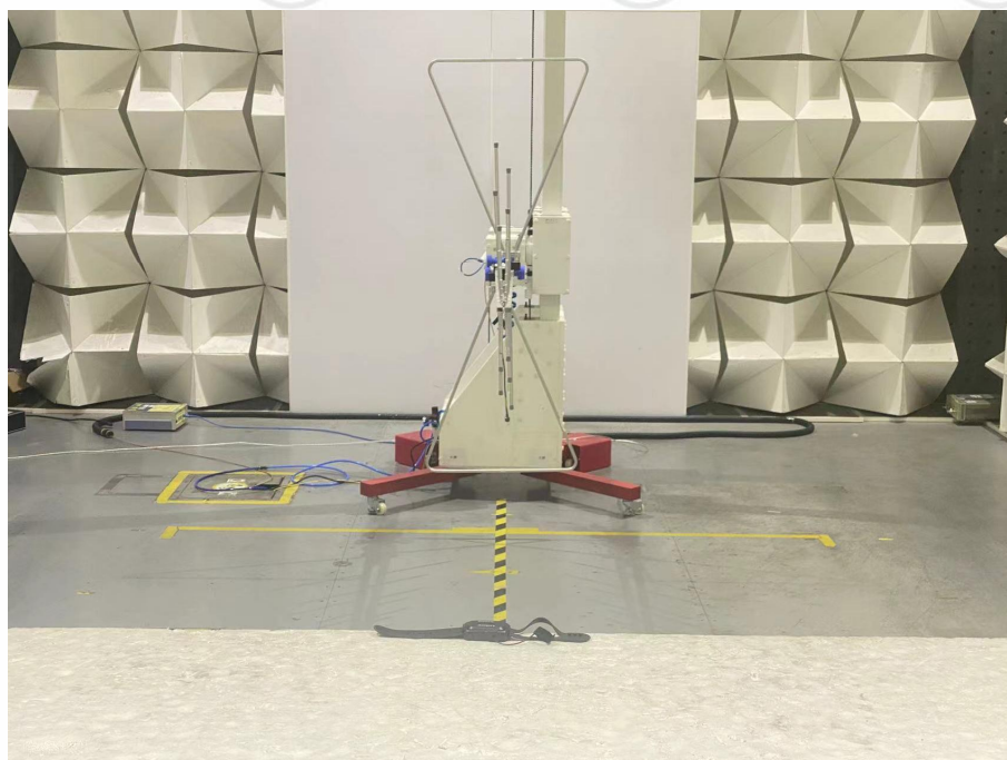
Radiated emission Test Setup-2 (30MHz~1GHz) close up photo
