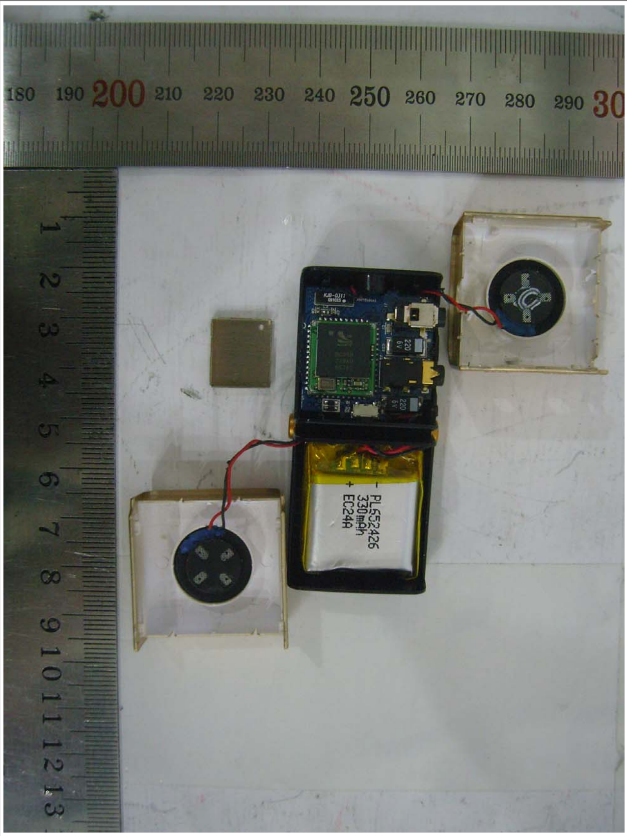
Internal view of EUT - Shield cover Remove state
