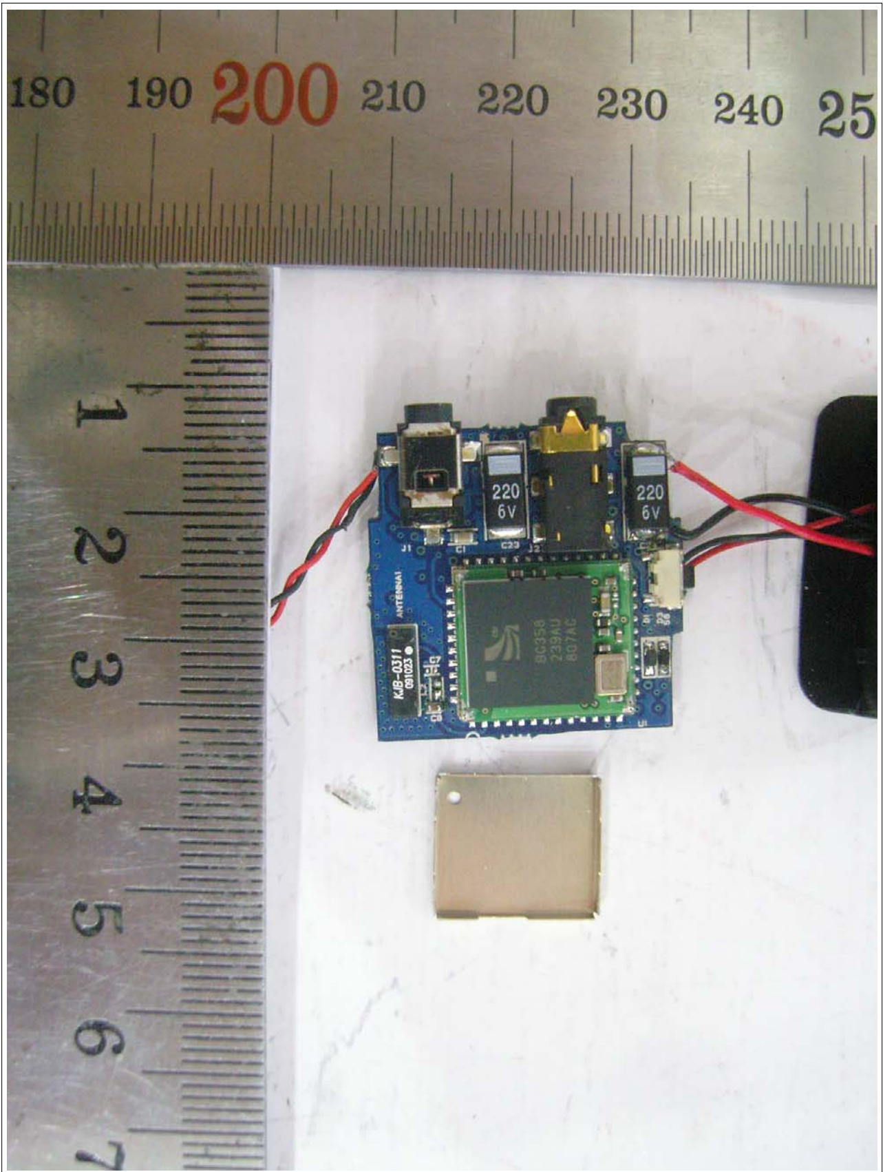
View of Main PCB(Top) - Shield cover Remove state
