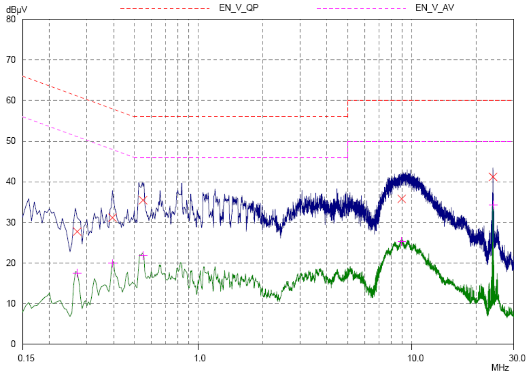
Figure 11. Plot of the Conducted Emissions
