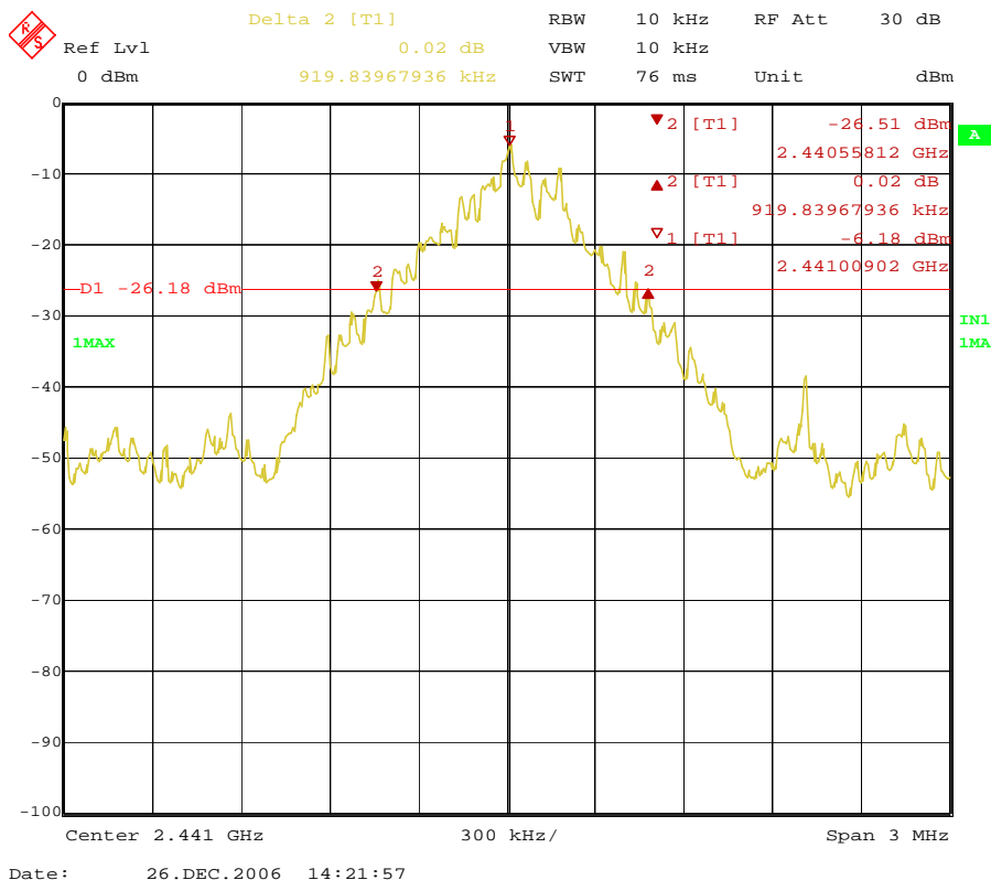
Middle Channel (operating at 2441 MHz)
