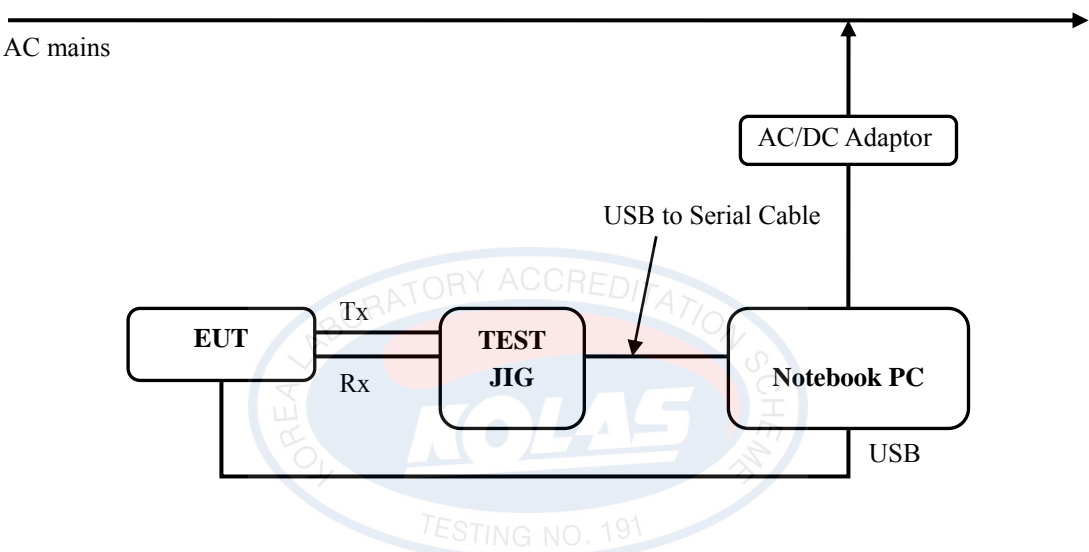
[ System Block Diagram of Test Configuration ]
