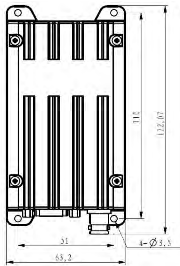
Fig.17 Top View
