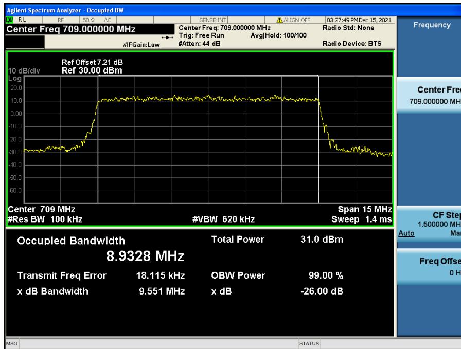
LTE Band 17 / 10 MHz / QPSK - RB Size 15
