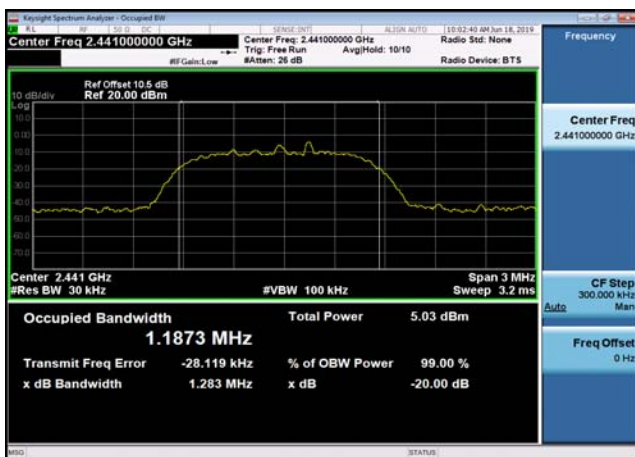
99% Bandwidth: DQPSK,2441MHz,2DH5
