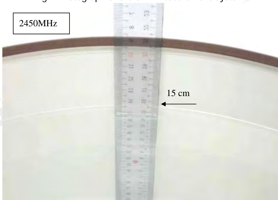
Fig.2 Photograph of the Tissue Simulant Fluid liquid depth 15cm for Flat (Body)
