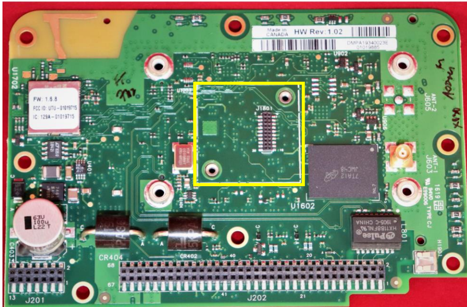
Figure 1 – PwrPak7-E2 (01010281) Bottom PCB
