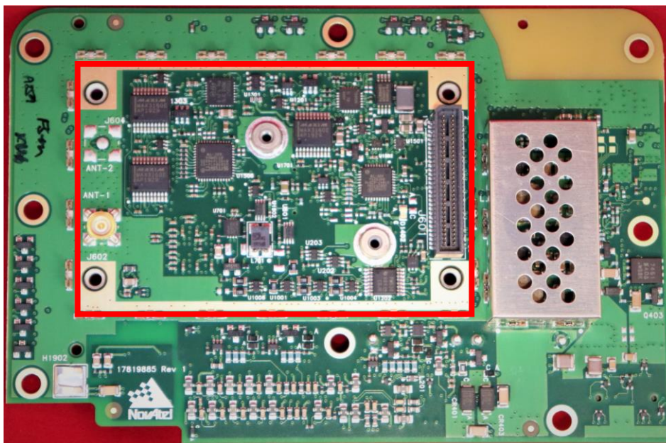
Figure 2 – PwrPak7-E2 (01010281) TOP PCB
