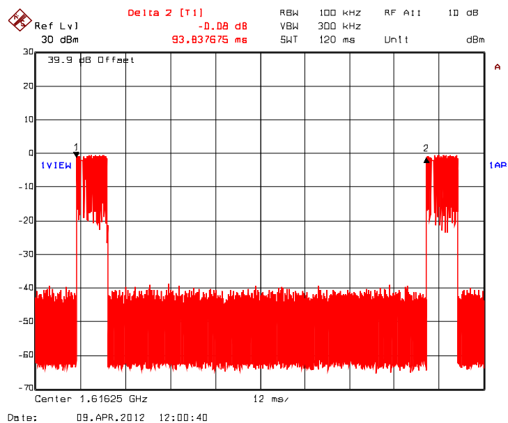
Plot 5.1.4.2. Duty Cycle, Period (93.84ms)
