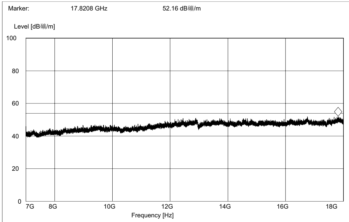
(Plot A.8: Antenna Vertical, 7GHz to 18GHz)
