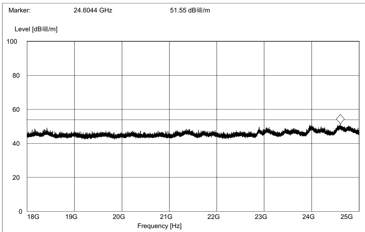
(Plot C.9: Antenna Vertical, 18GHz to 25GHz)
