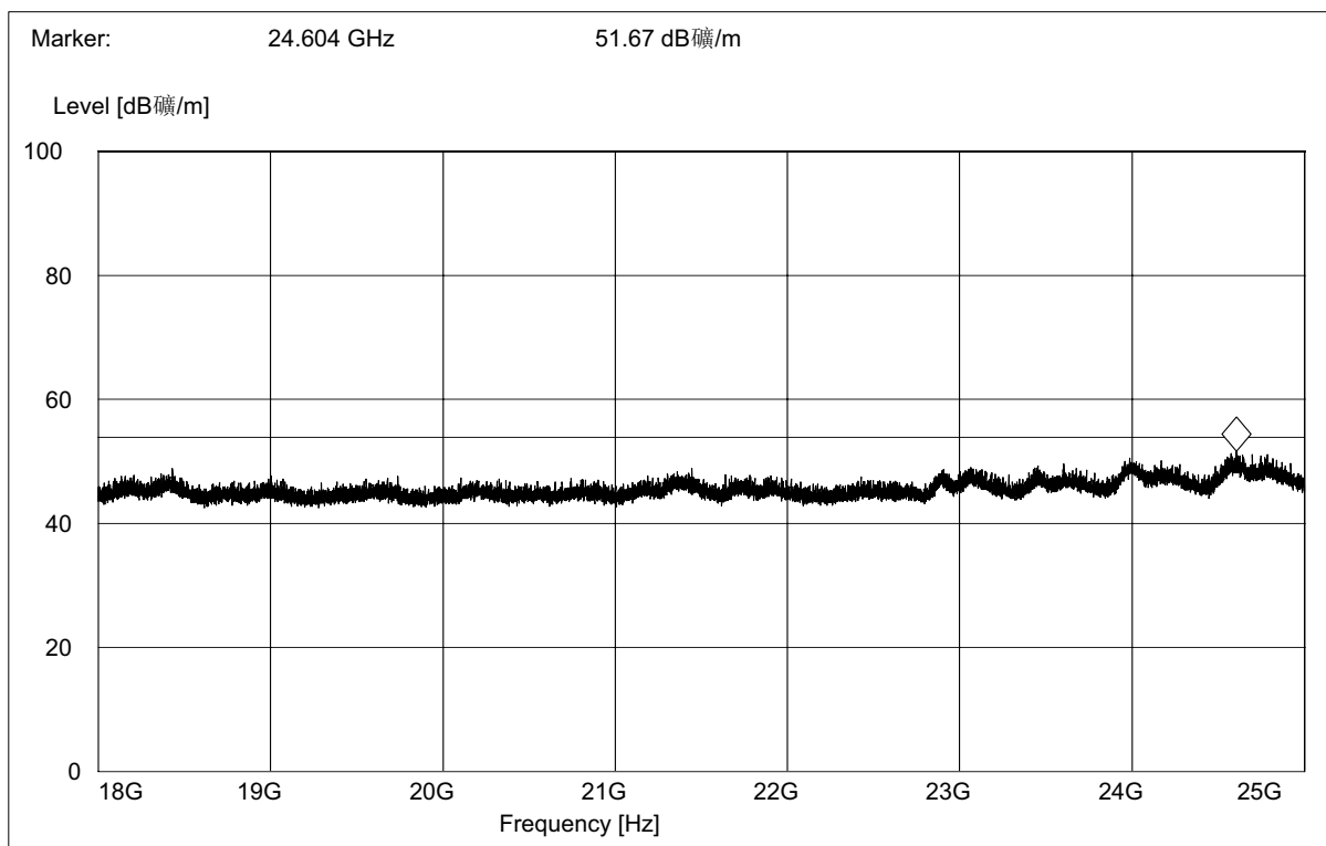
(Plot C.5: Antenna Horizontal, 18GHz to 25GHz)
