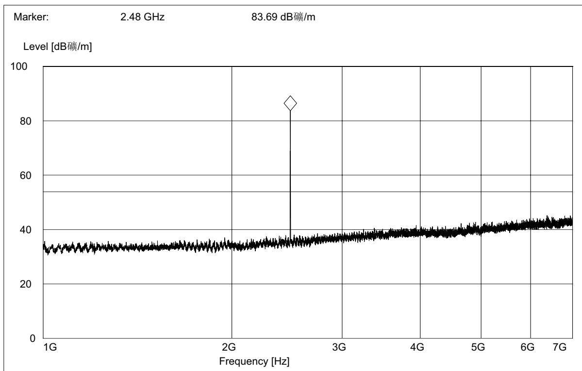
(Plot C.3: Antenna Horizontal, 1GHz to 7GHz)
