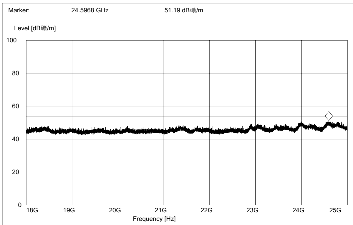
(Plot A.5: Antenna Horizontal, 18GHz to 25GHz)
