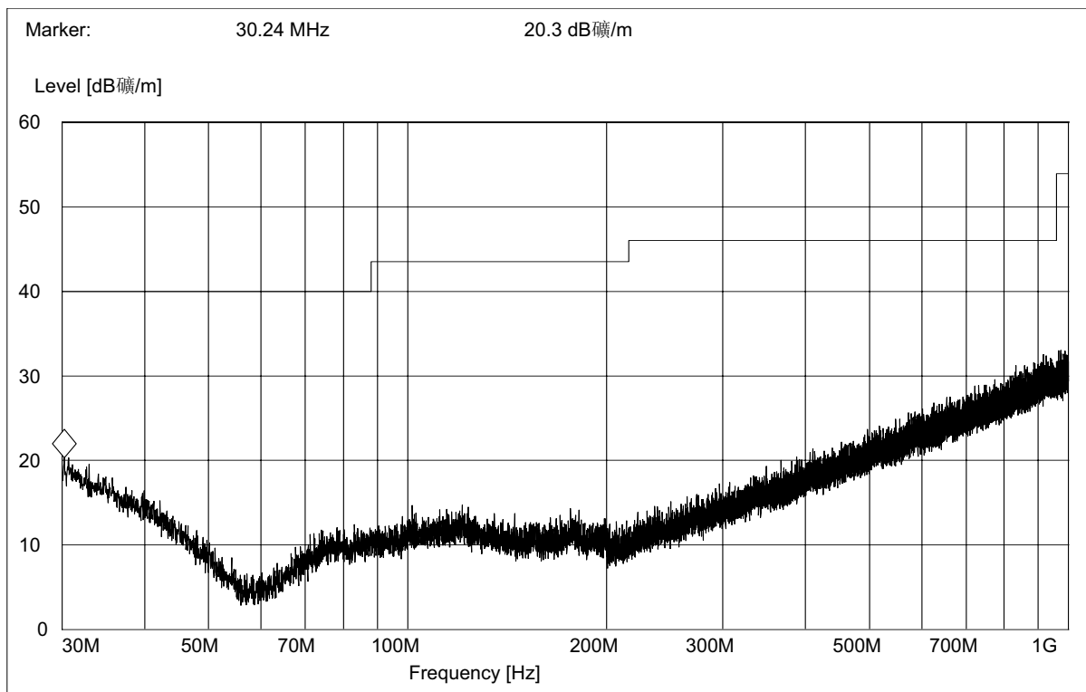
(Plot B.2: Antenna Horizontal, 30MHz to 1GHz)
