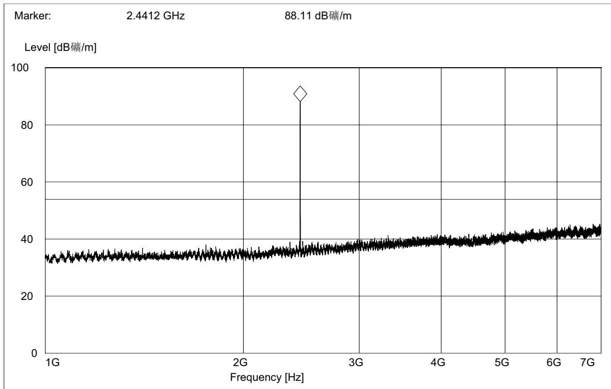
(Plot B.7: Antenna Vertical, 1GHz to 7GHz)
