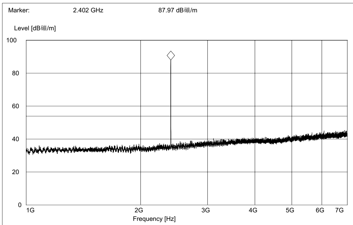
(Plot A.7: Antenna Vertical, 1GHz to 7GHz)
