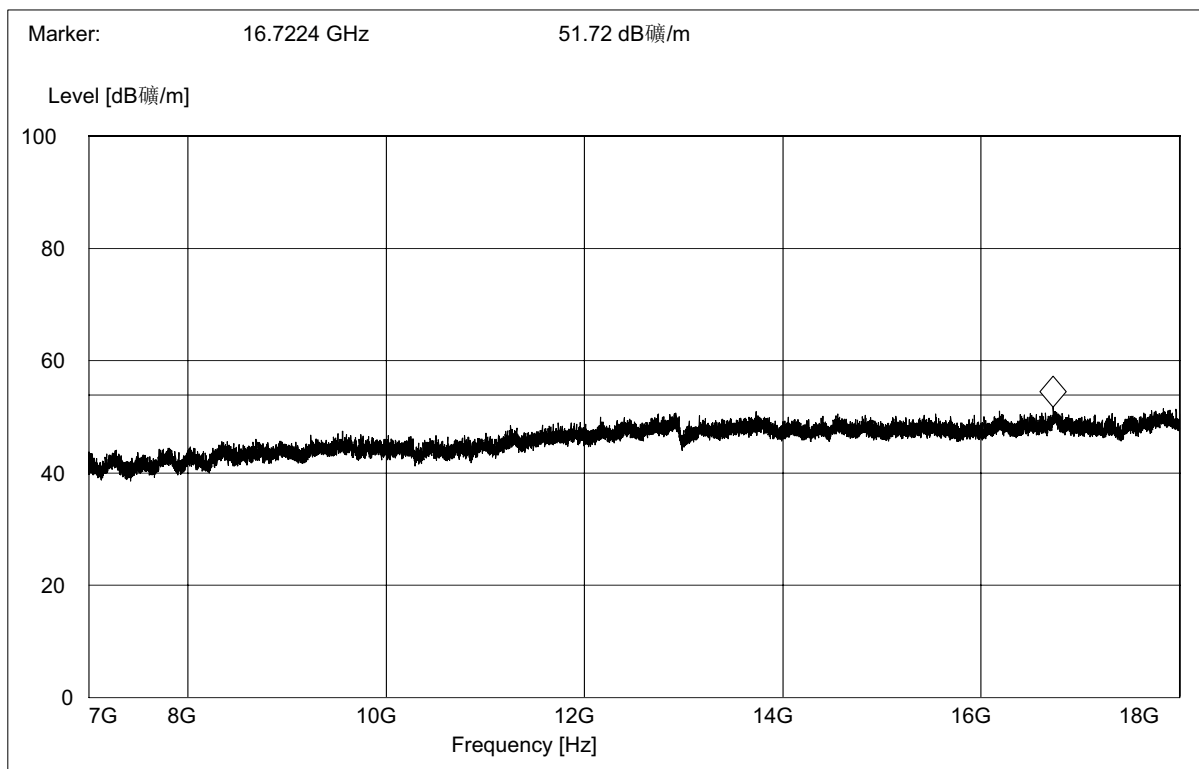
(Plot B.4: Antenna Horizontal, 7GHz to 18GHz)
