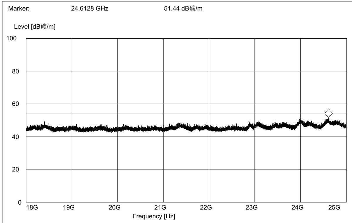
(Plot B.9: Antenna Vertical, 18GHz to 25GHz)
