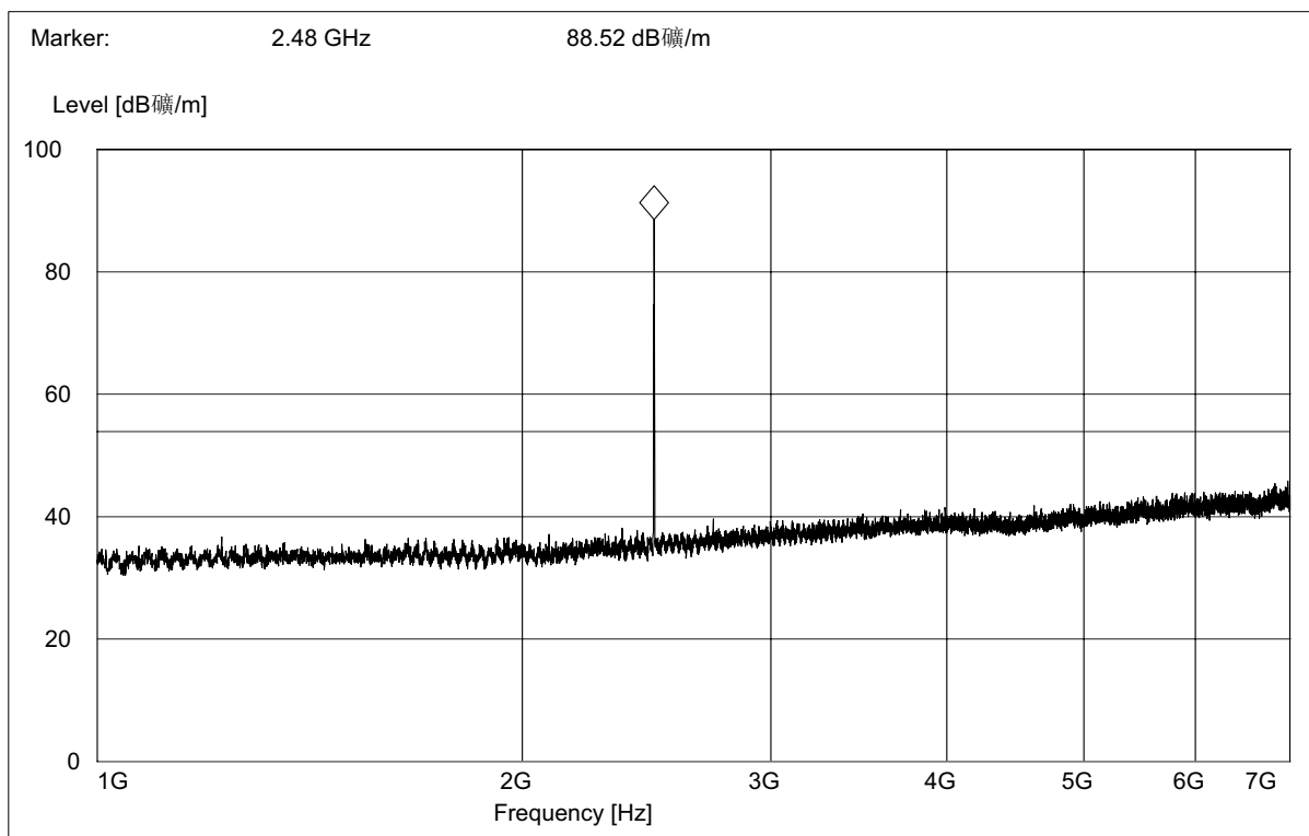
(Plot C.7: Antenna Vertical, 1GHz to 7GHz)
