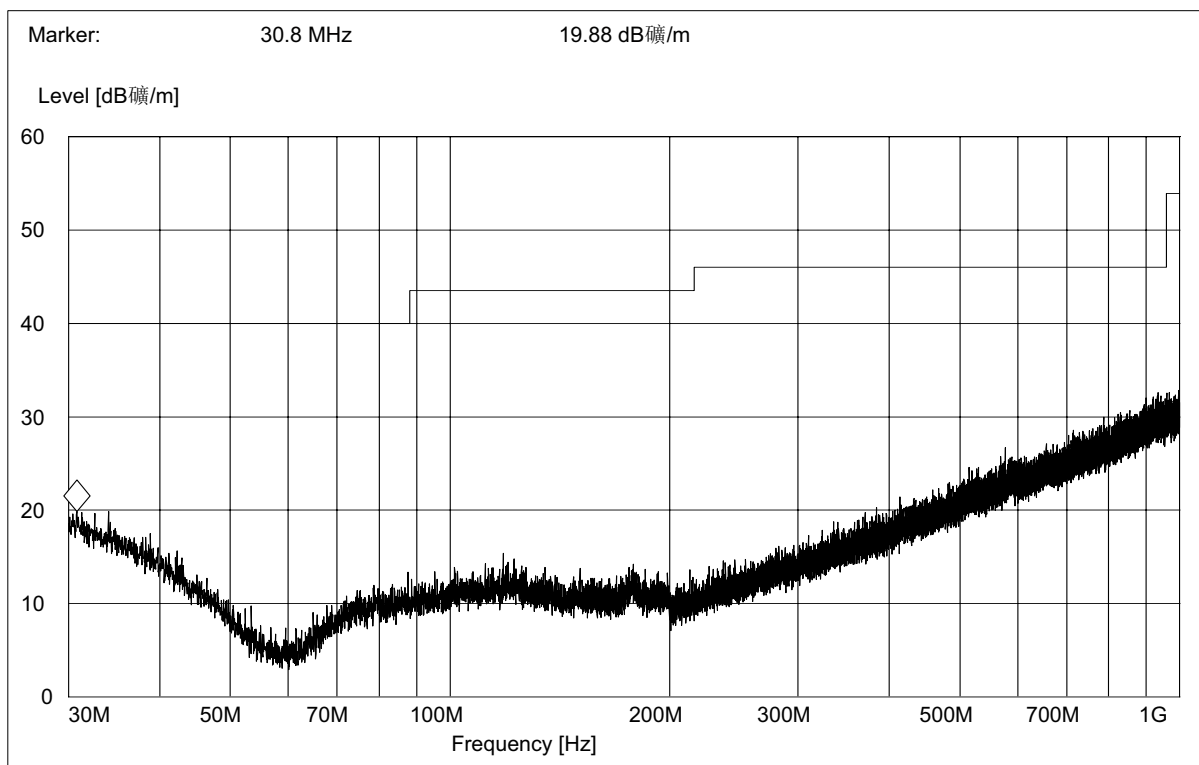
(Plot B.6: Antenna Vertical, 30MHz to 1GHz)
