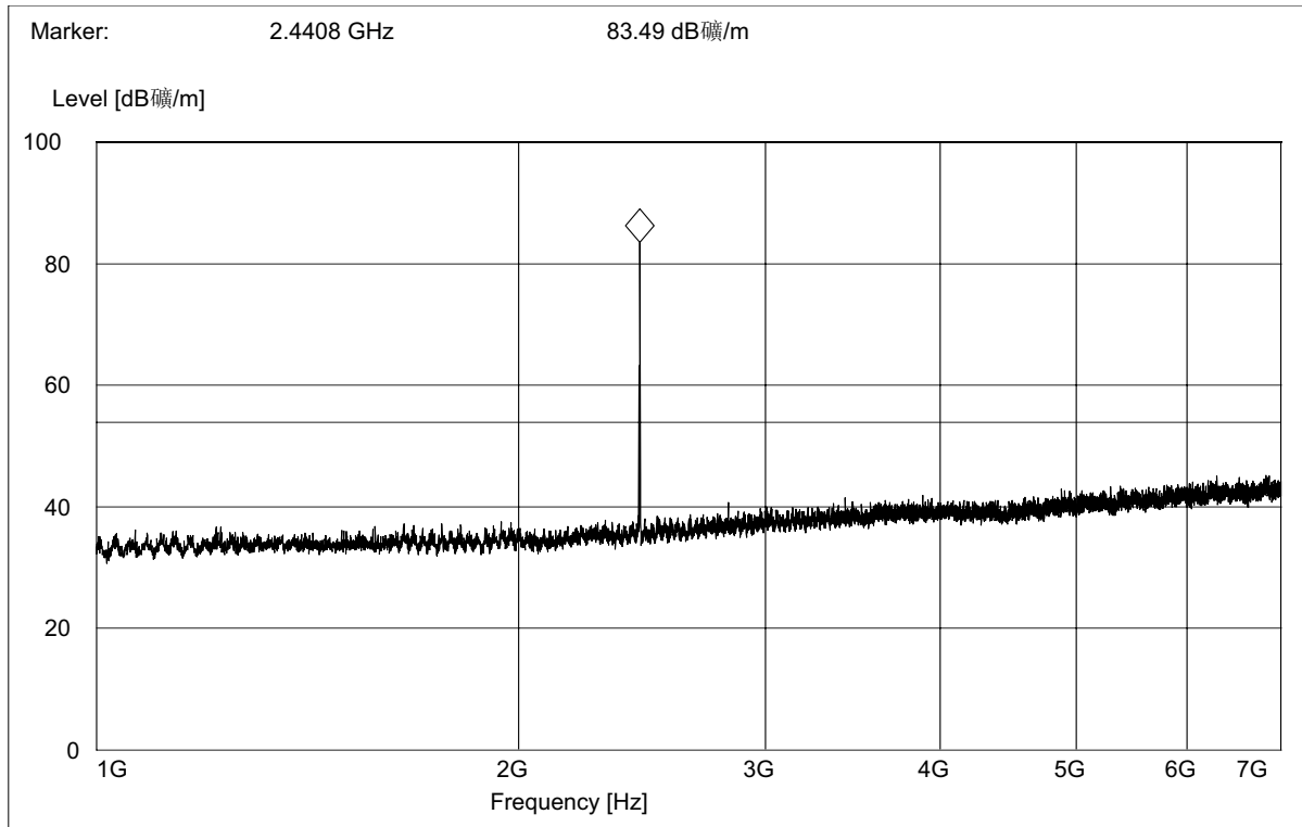
(Plot B.3: Antenna Horizontal, 1GHz to 7GHz)
