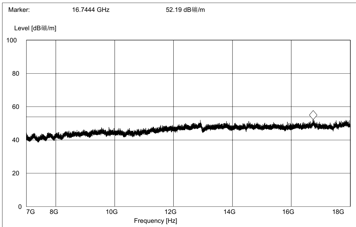
(Plot B.8: Antenna Vertical, 7GHz to 18GHz)
