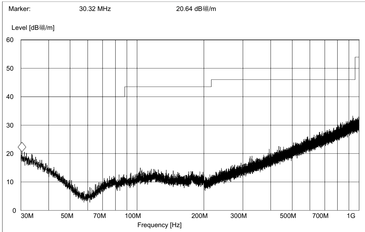
(Plot A.2: Antenna Horizontal, 30MHz to 1GHz)
