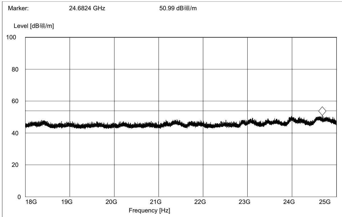
(Plot B.5: Antenna Horizontal, 18GHz to 25GHz)
