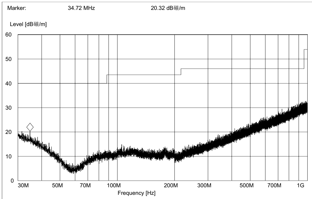
(Plot C.6: Antenna Vertical, 30MHz to 1GHz)
