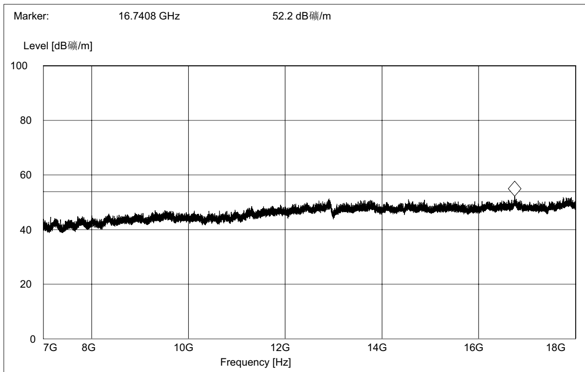
(Plot C.8: Antenna Vertical, 7GHz to 18GHz)
