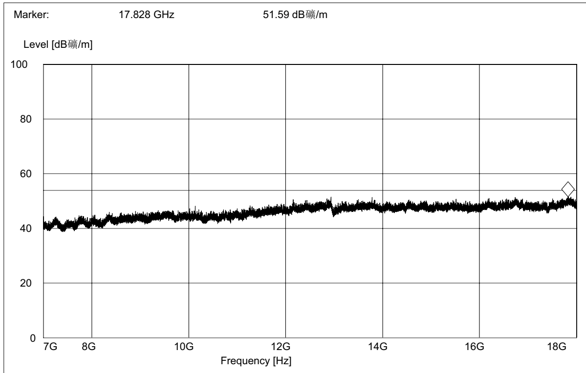
(Plot A.4: Antenna Horizontal, 7GHz to 18GHz)
