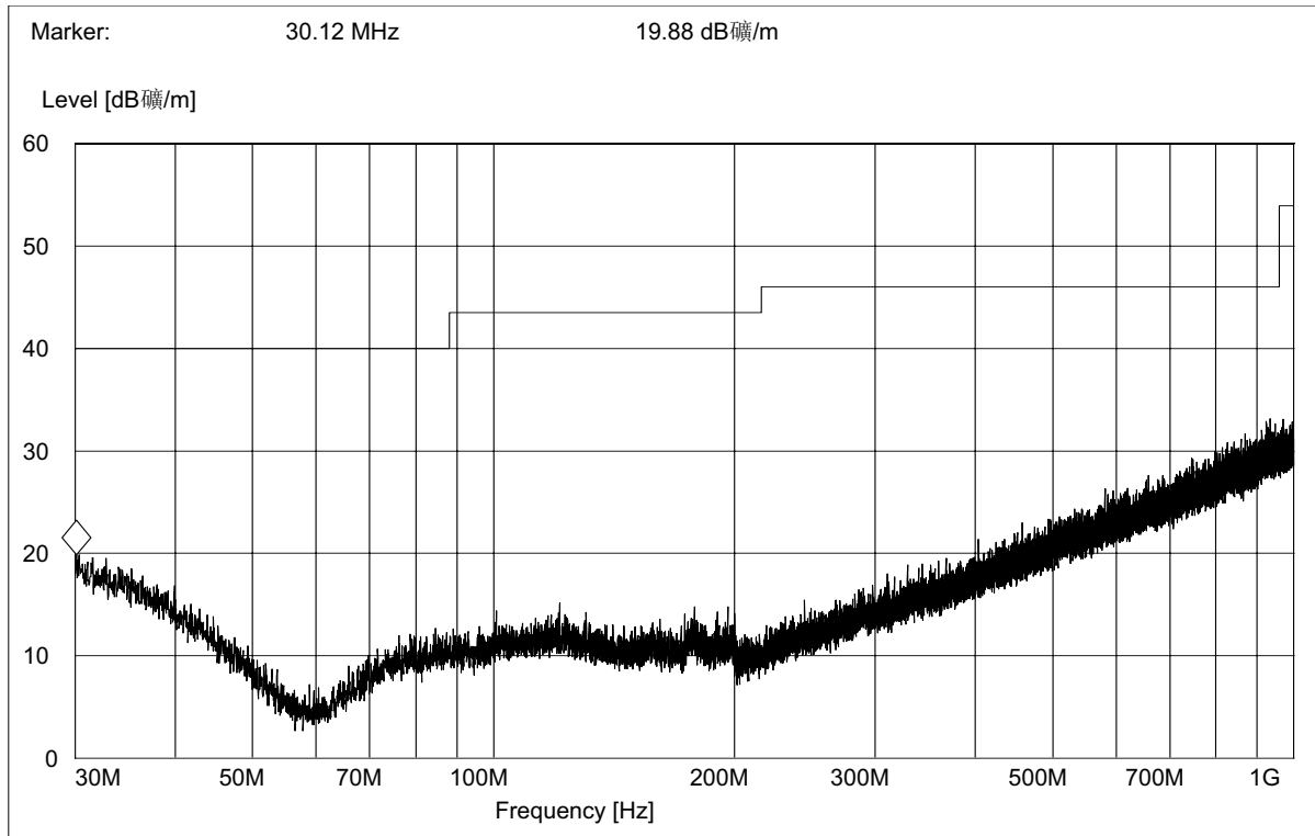
(Plot A.6: Antenna Vertical, 30MHz to 1GHz)
