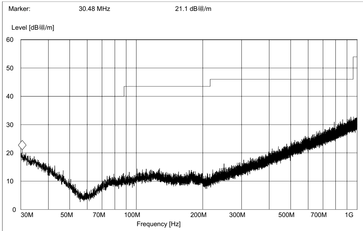
(Plot C.2: Antenna Horizontal, 30MHz to 1GHz)
