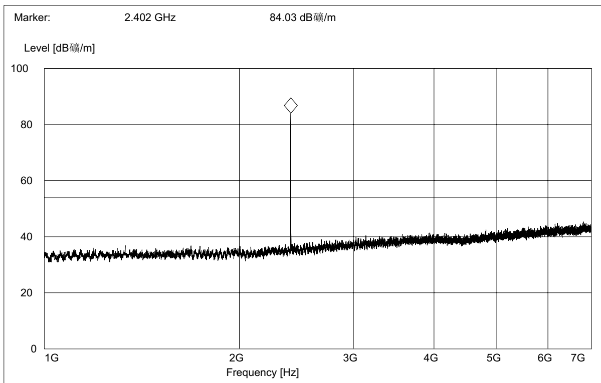
(Plot A.3: Antenna Horizontal, 1GHz to 7GHz)
