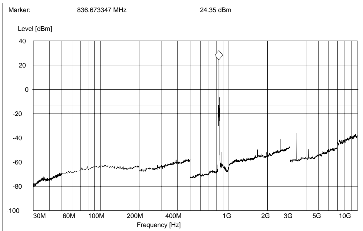
(Plot B.2: Channel = 190, Test Antenna Vertical)
