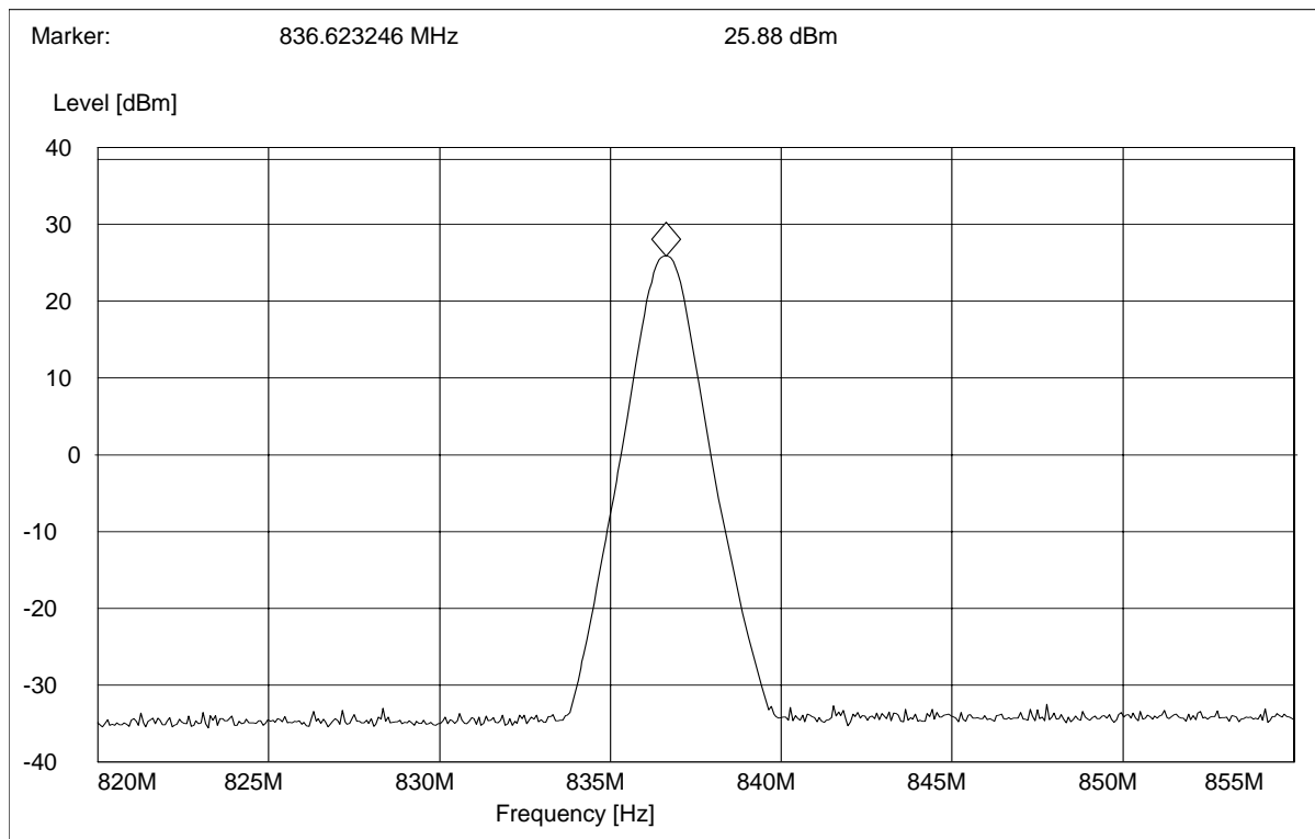
(Plot B: Channel = 190)
