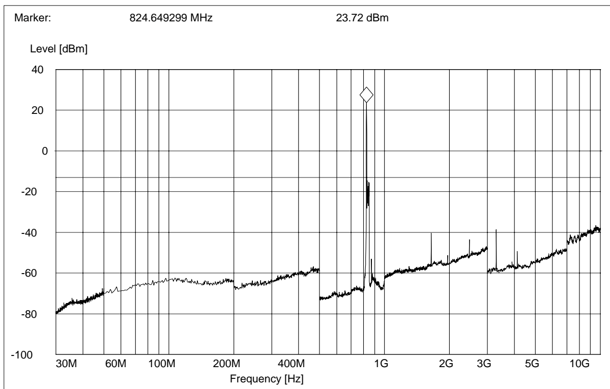
(Plot A.2: Channel = 128, Test Antenna Vertical)
