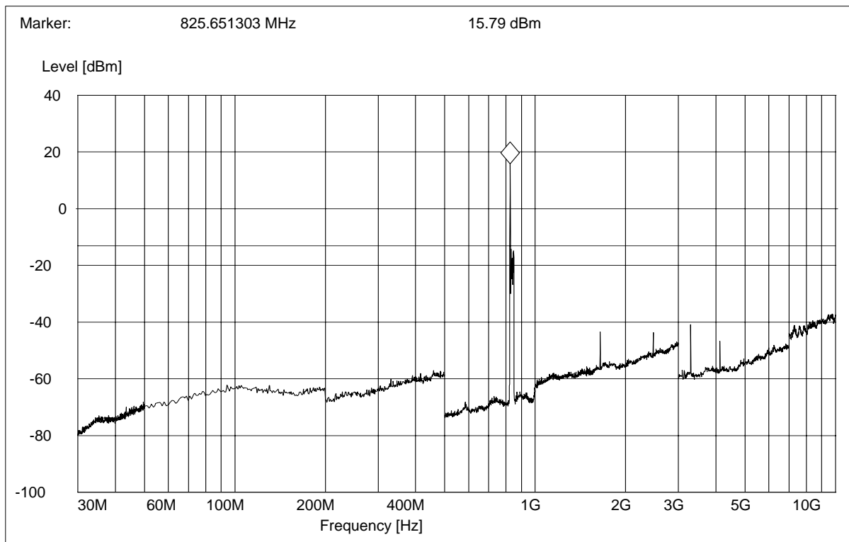
(Plot A.1: Channel = 128, Test Antenna Horizontal)
