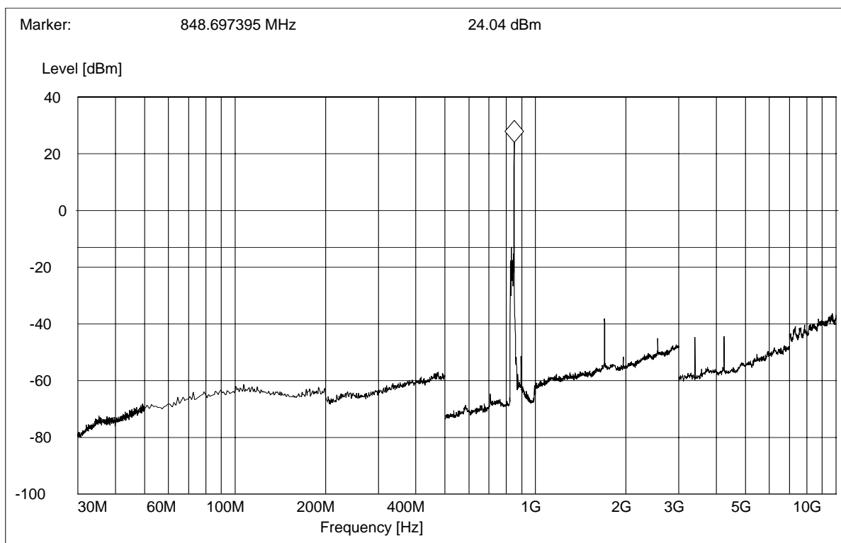
(Plot C.2: Channel = 251, Test Antenna Vertical)
