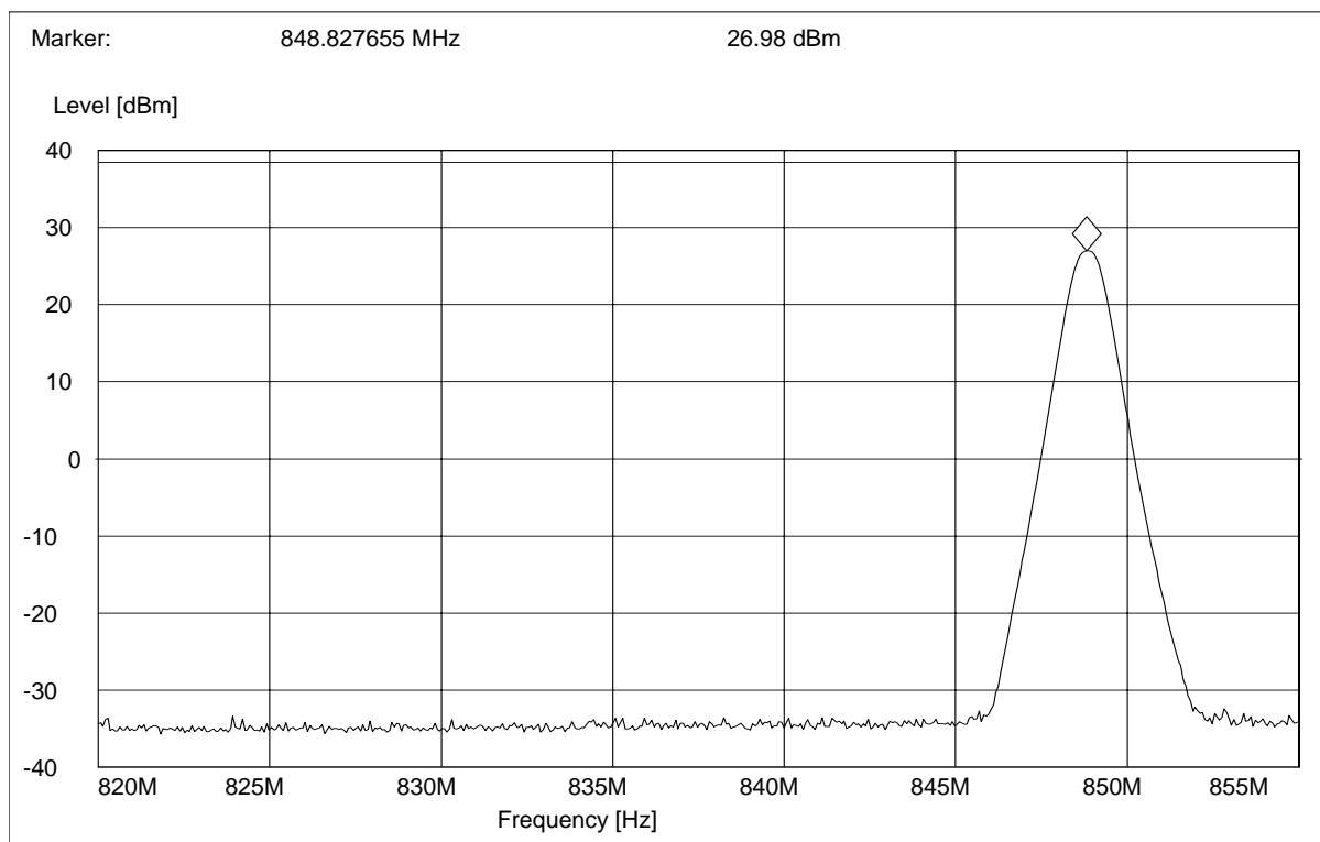
(Plot C: Channel = 251)
