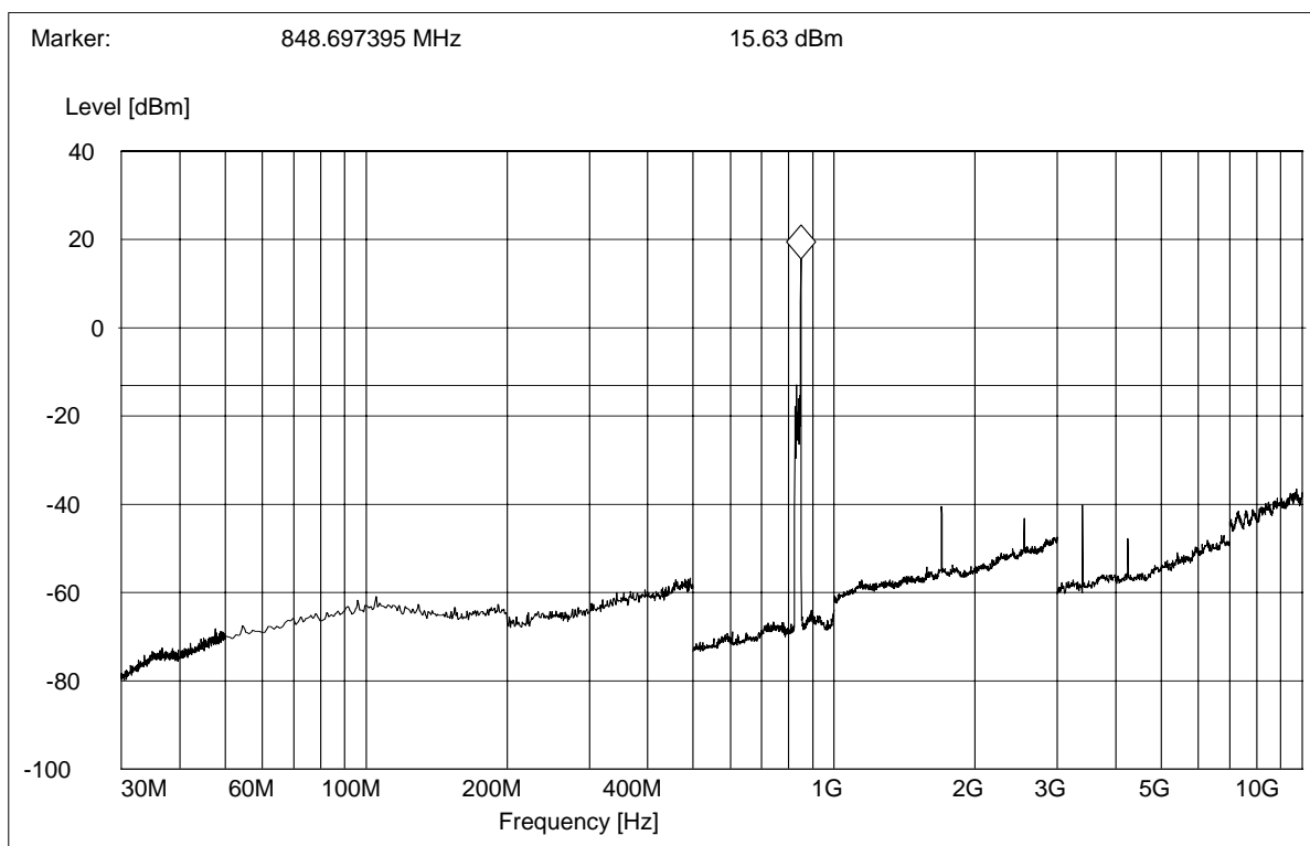
(Plot C.1: Channel = 251, Test Antenna Horizontal)
