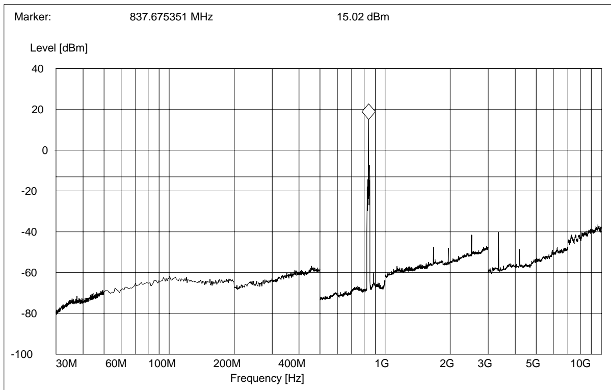
(Plot B.1: Channel = 190, Test Antenna Horizontal)
