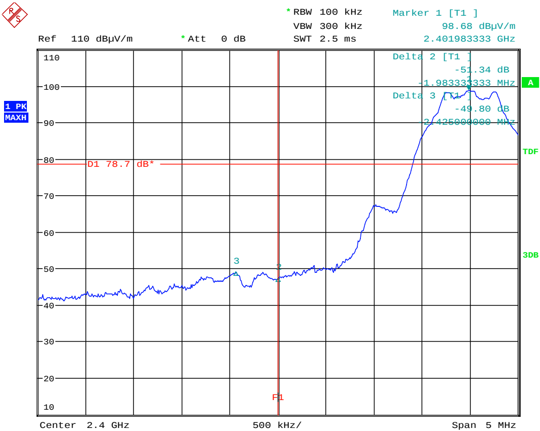
Lower Bandedge compliance
