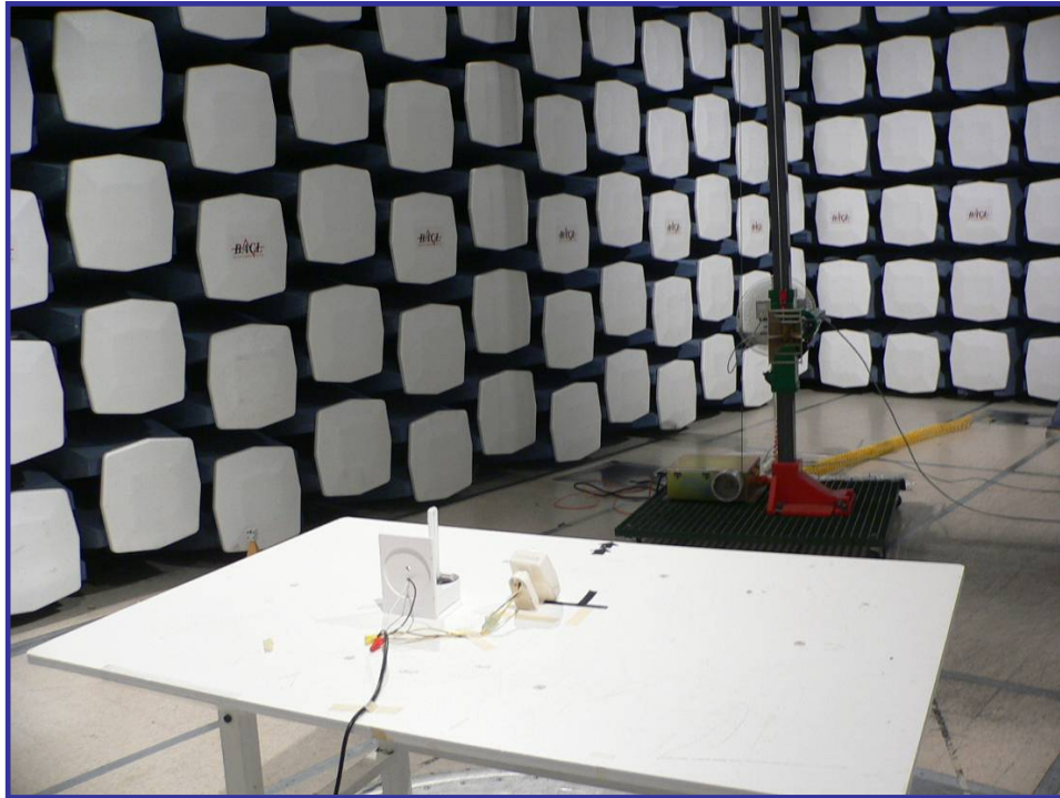
Radiated Emissions: 18 GHz to 26.5GHz – Rear View
