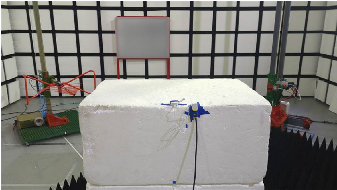
RADIATED ABOVE 1GHz BACK
