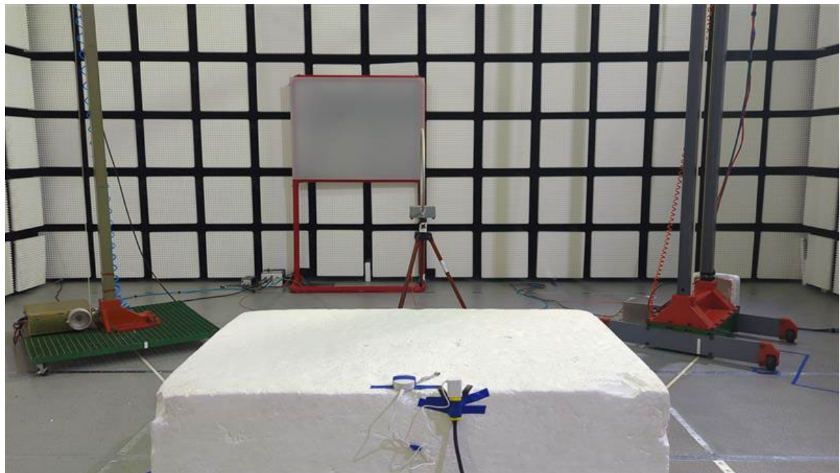
RADIATED BELOW 30MHz 90 DEG
