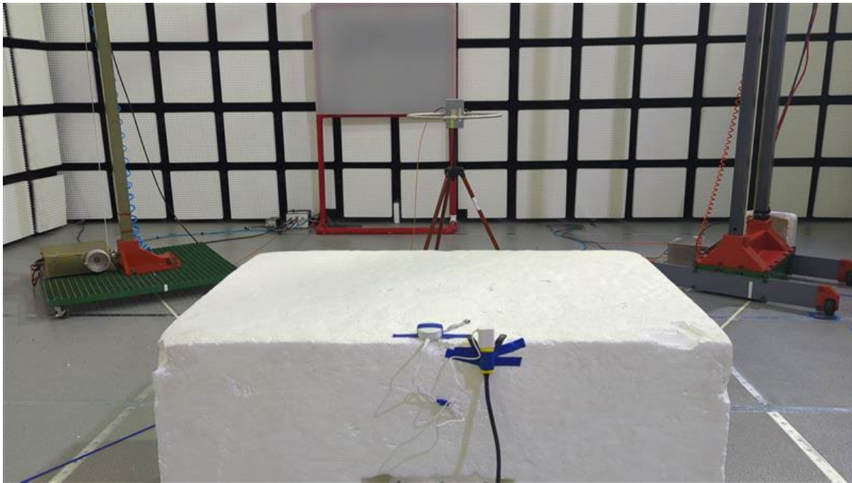
RADIATED BELOW 30MHz FLAT
