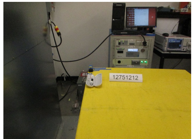
AC LINE CHARGING BACK PHOTO
