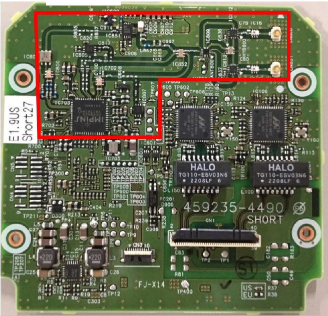
RF circuit
