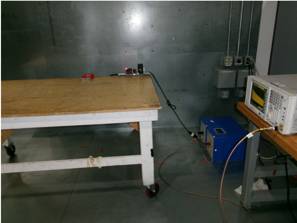
Lock Off (LED Red) CEMI Set up
