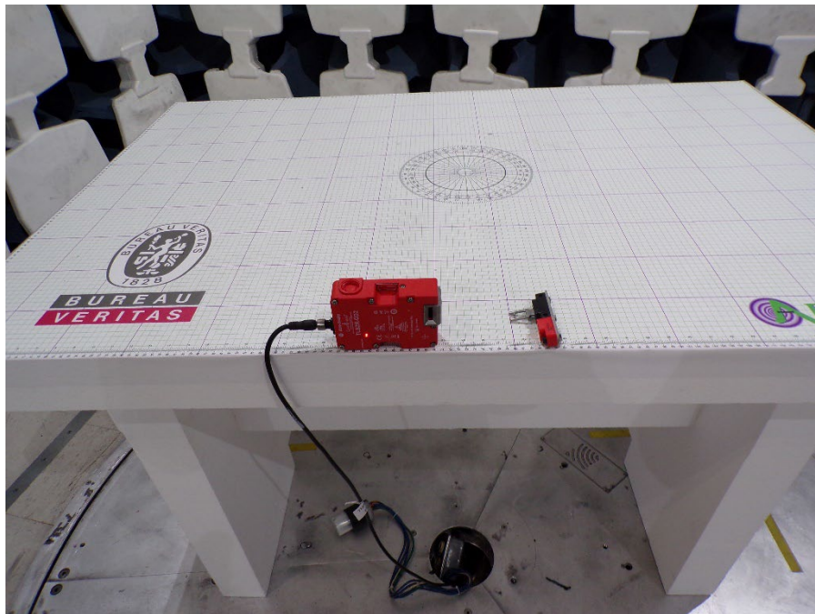
Y-Axis 30-1000MHz Lock OFF (LED Red)
