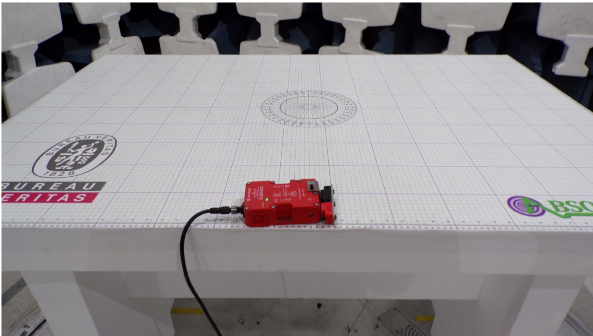
X-Axis 0.009-30MHz Lock ON (LED Green – Actuator Position 1)
