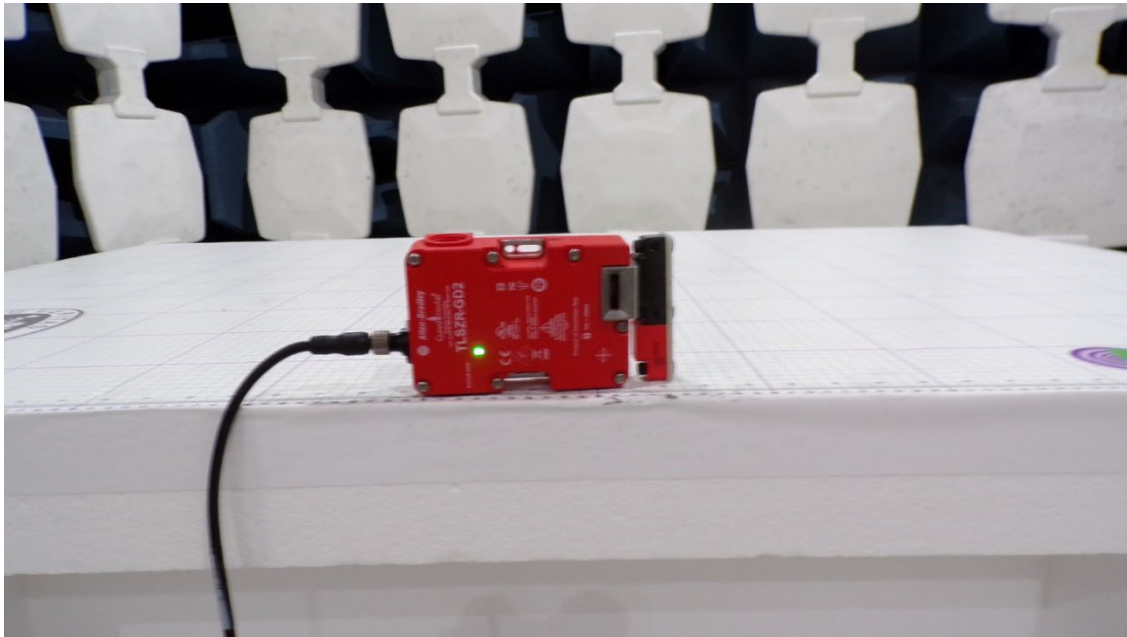
Y-Axis 30-1000MHz Lock ON (LED Green – Actuator Position 1)
