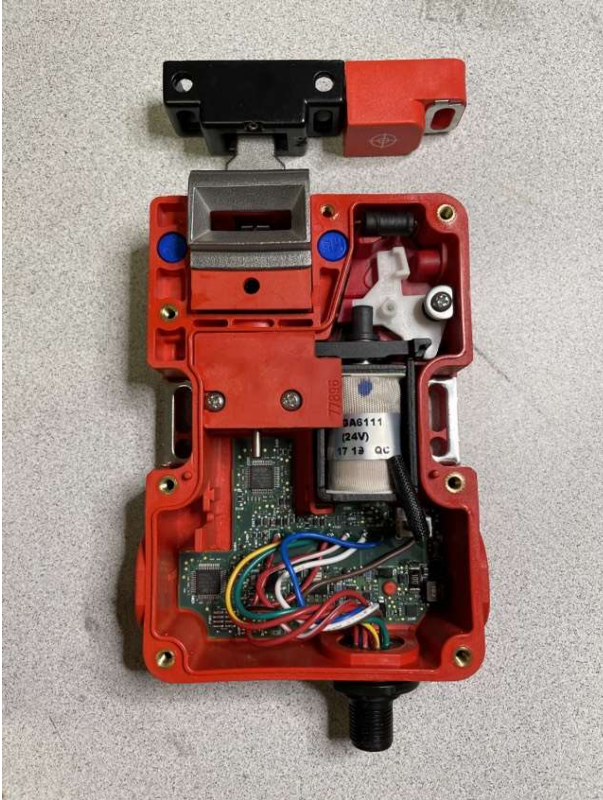
Fig 1. Internal View
