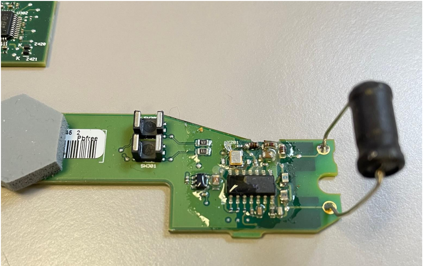
Fig 6. TLS-Z Ser. F PCB RFID Circuit – 3
