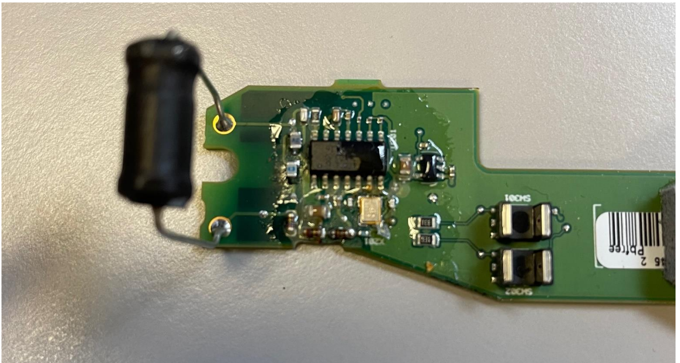
Fig 4. TLS-Z Ser. F PCB RFID Circuit – 1
