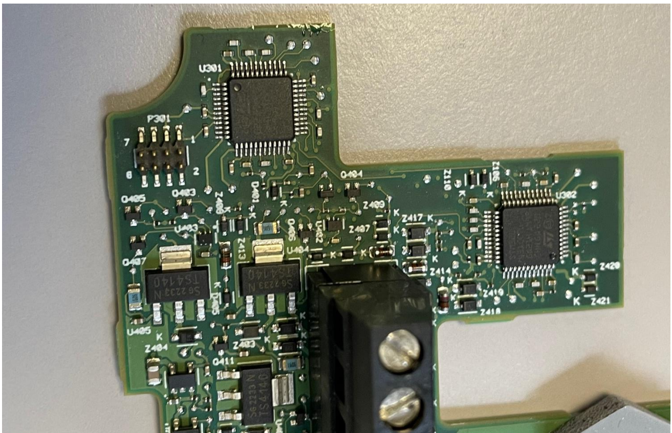
Fig 7. TLS-Z Ser. F PCB MCU Top View
