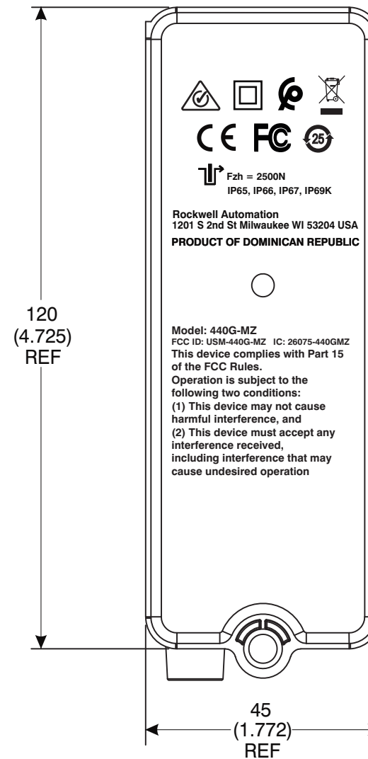
BOTTOM VIEW OF HOUSING
