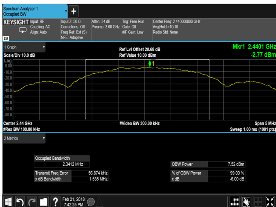
Figure 2 - 2440 MHz – 6 dB Bandwidth & 99% Occupied Bandwidth
