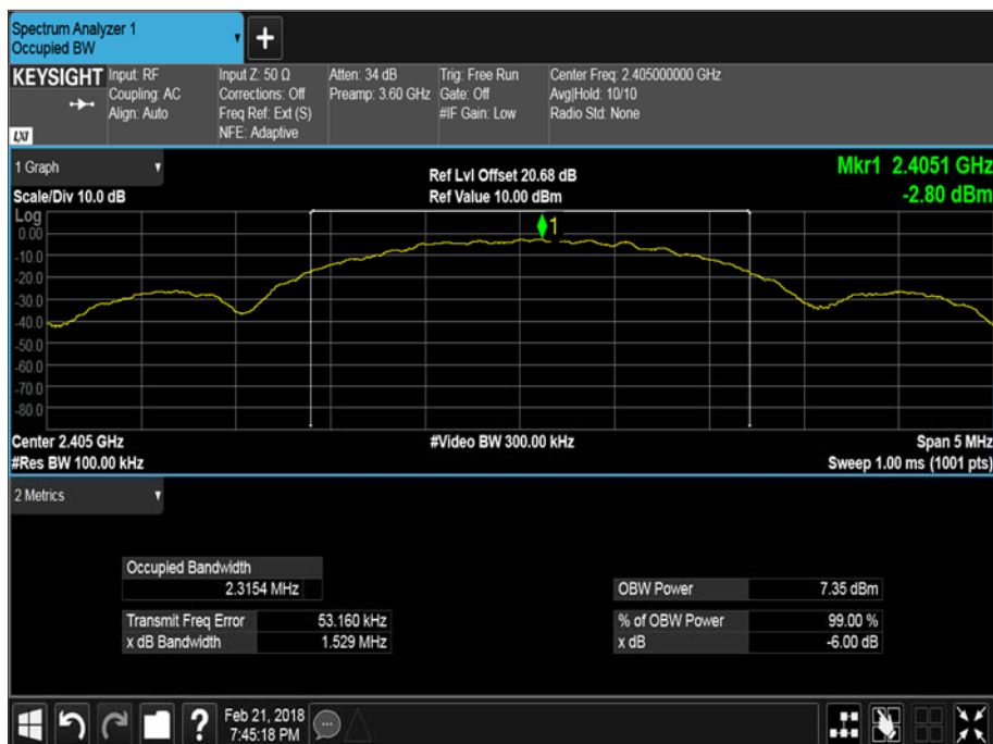
Figure 1 - 2405 MHz – 6 dB Bandwidth & 99% Occupied Bandwidth
