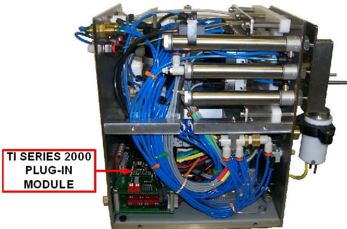
Processing Unit – Left Side View
