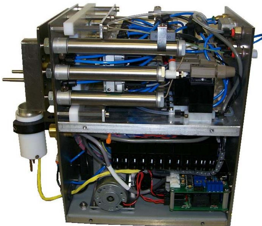
Processing Unit – Right Side View
