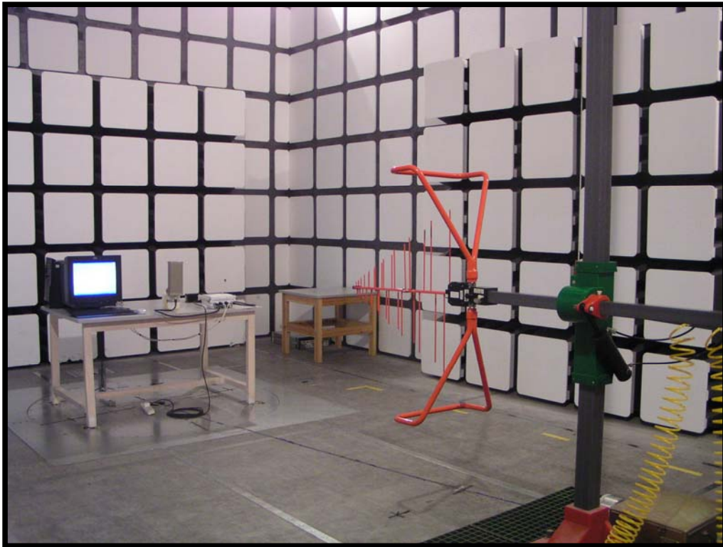
Radiated Emissions - Rear View (30-1000MHz) for 802.11a directional Antenna (Antenna Mode: TQWTD-1700-5.5V)
