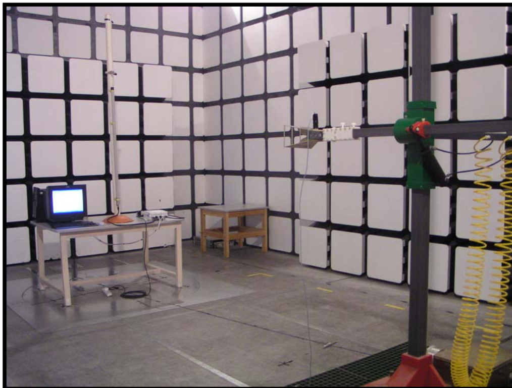
Radiated Emissions - Rear View (Above 1GHz) for 802.11b/g 12 dBi Omni Antenna (Antenna model: XPTX2412-QX)
