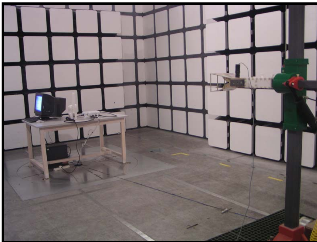
Radiated Emissions – Rear View (Above 1GHz) for 802.11b/g 11 dBi Directional Antenna (Antenna model: SPDG14T)
