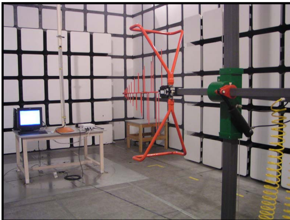
Radiated Emissions - Rear View (30-1000MHz) for 802.11b/g 12 dBi Omni Antenna (Antenna model: XPTX2412-QX)
