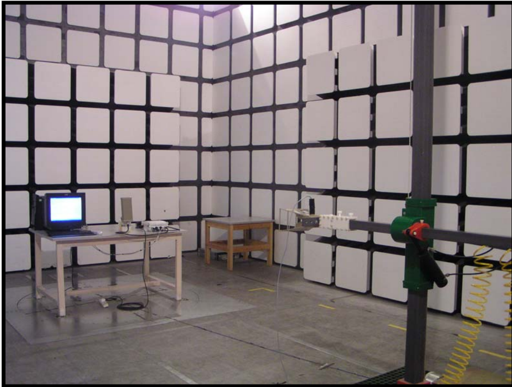
Radiated Emissions - Rear View (Above 1GHz) for 802.11a directional Antenna (Antenna Mode: TQWTD-1700-5.5V)
