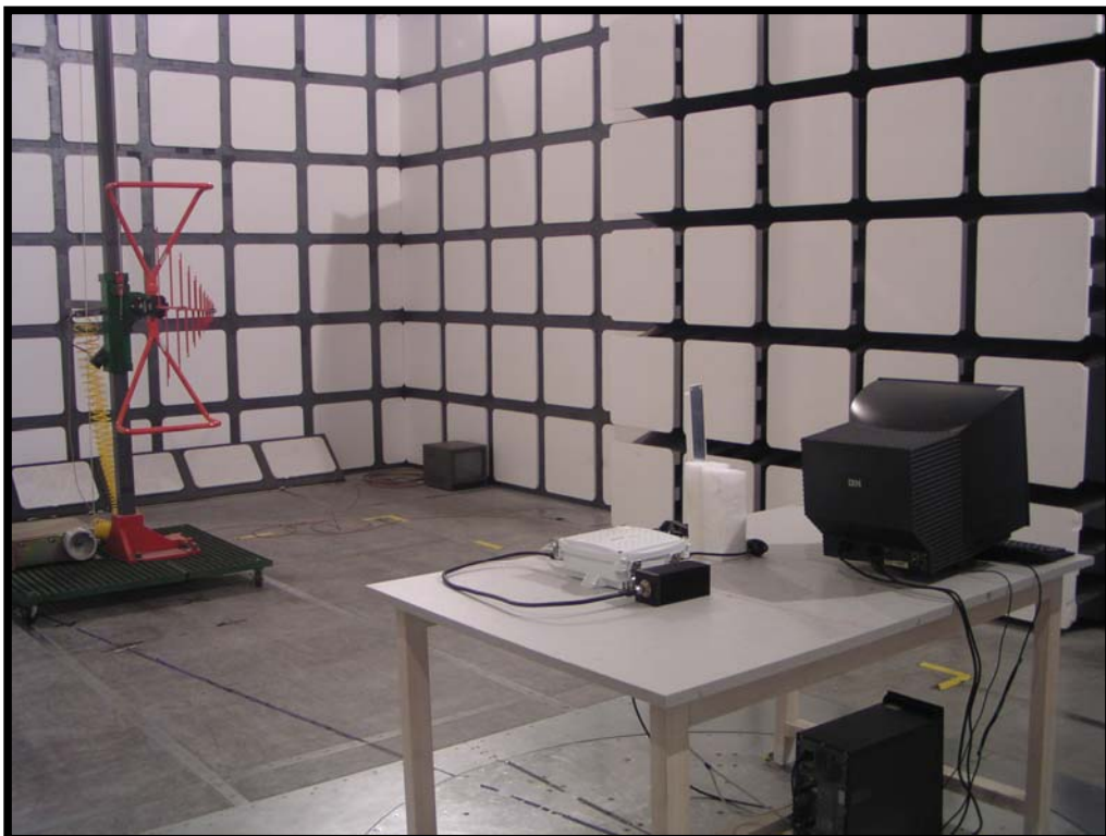
Radiated Emissions - Rear View (30-1000MHz) for 802.11b/g 11 dBi Directional Antenna (Antenna model: SPDG14T)
