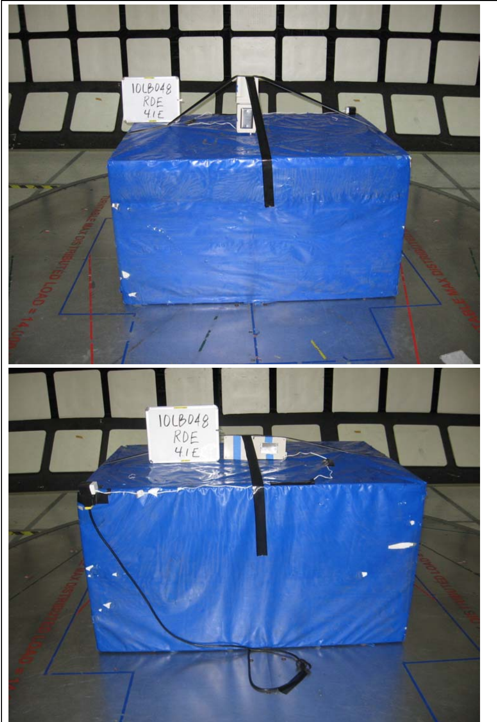
Figure 1 Test setup photo for Radiated Emissions (Reader, X and Y Orientations)
