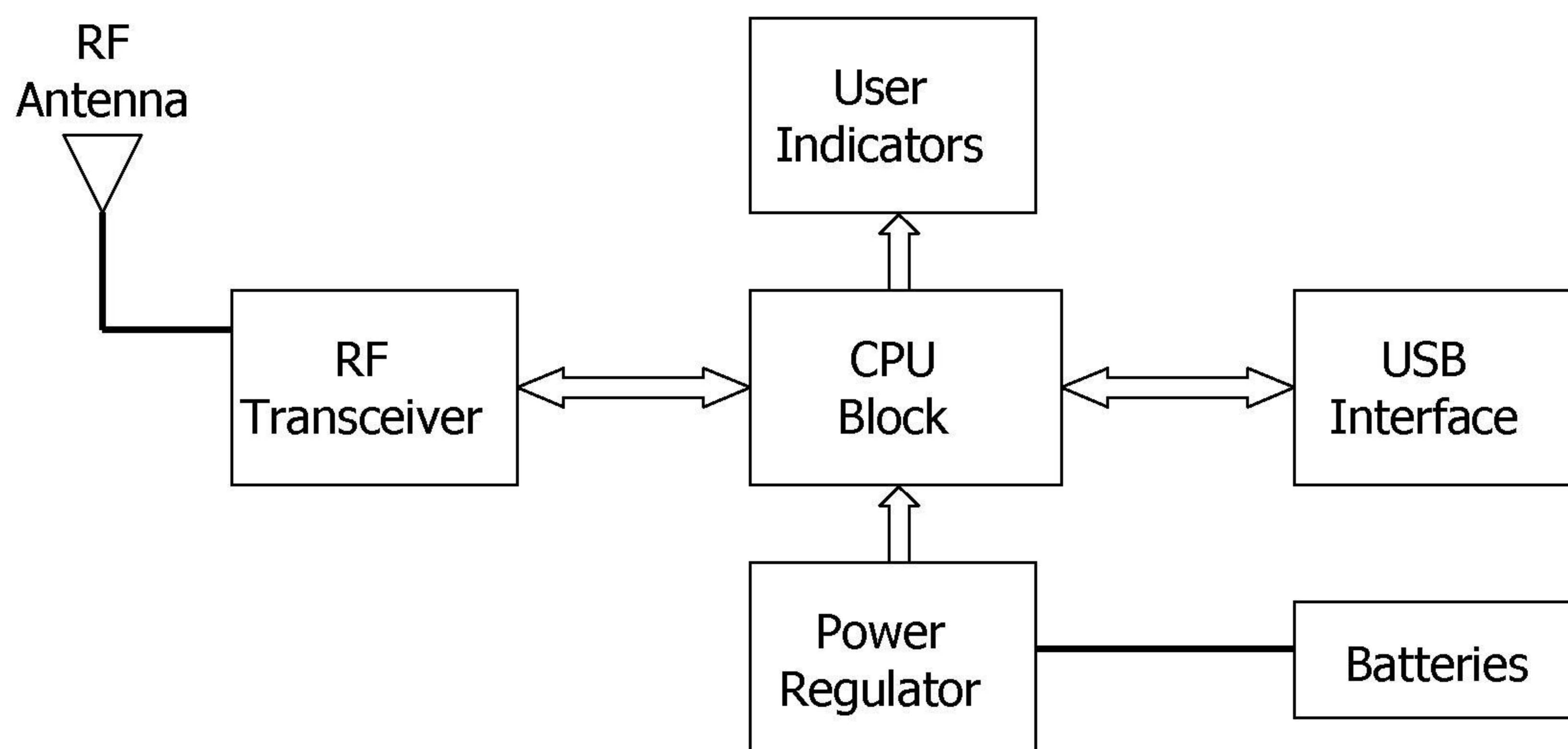
Remote Controller (DL1) Block Diagram
