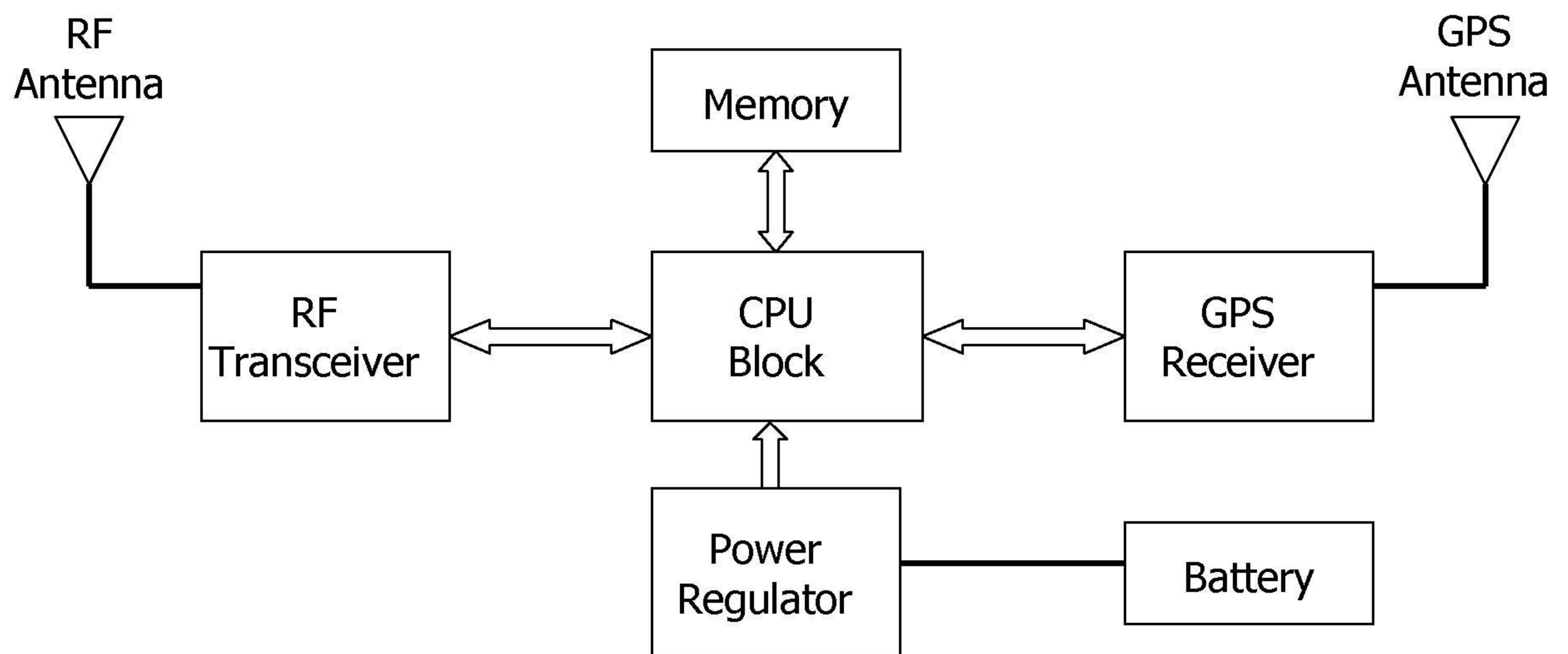
Main Unit (T3) Block Diagram
