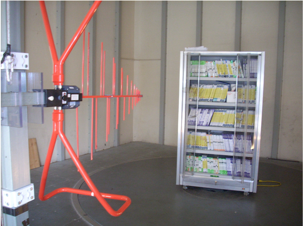
Spurious emissions above 30MHz
