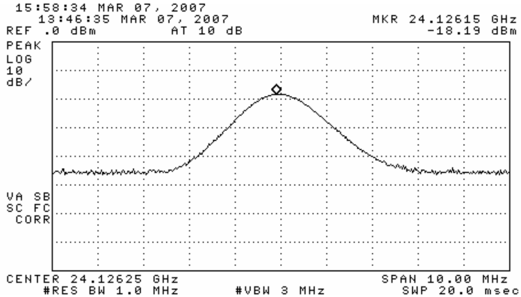
Figure 6.1. Fundamental spectrum. (3 meters, peak hold)
