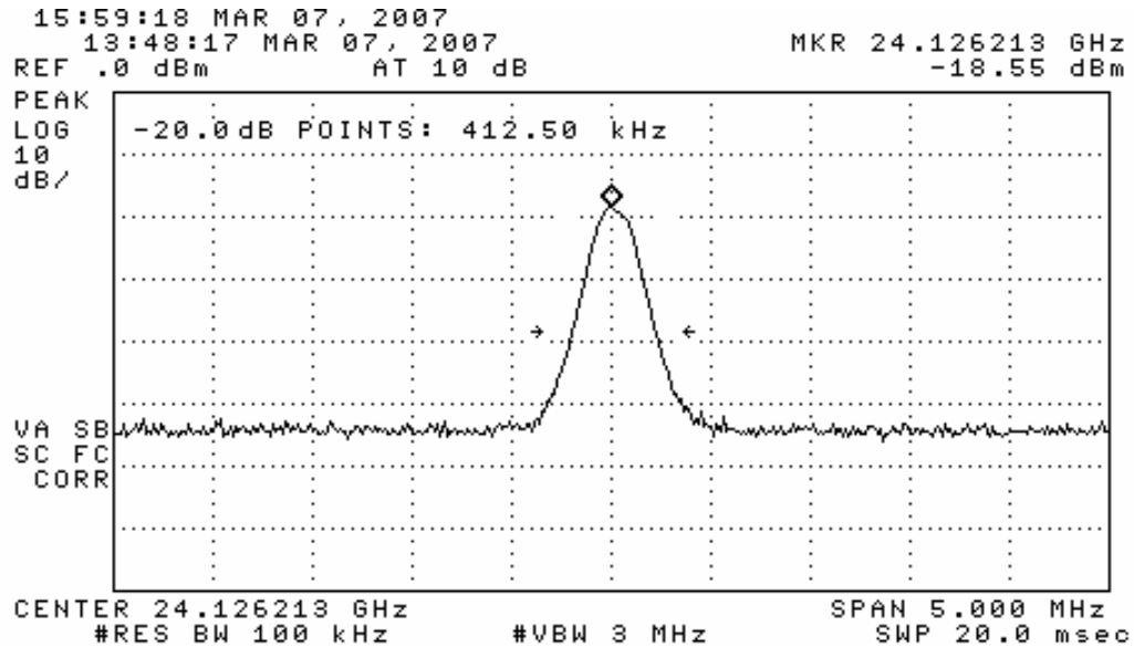
Figure 6.2. Fundamental Bandwidth Measurement.
