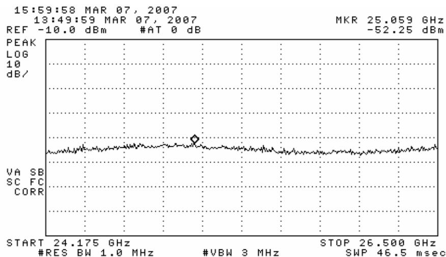
Figure 6.3. Digital/Spurious Emissions. (top) 30-1000 MHz, (middle) 22-24.075 GHz - noise, (bottom) 24.175-26.5 GHz - noise
