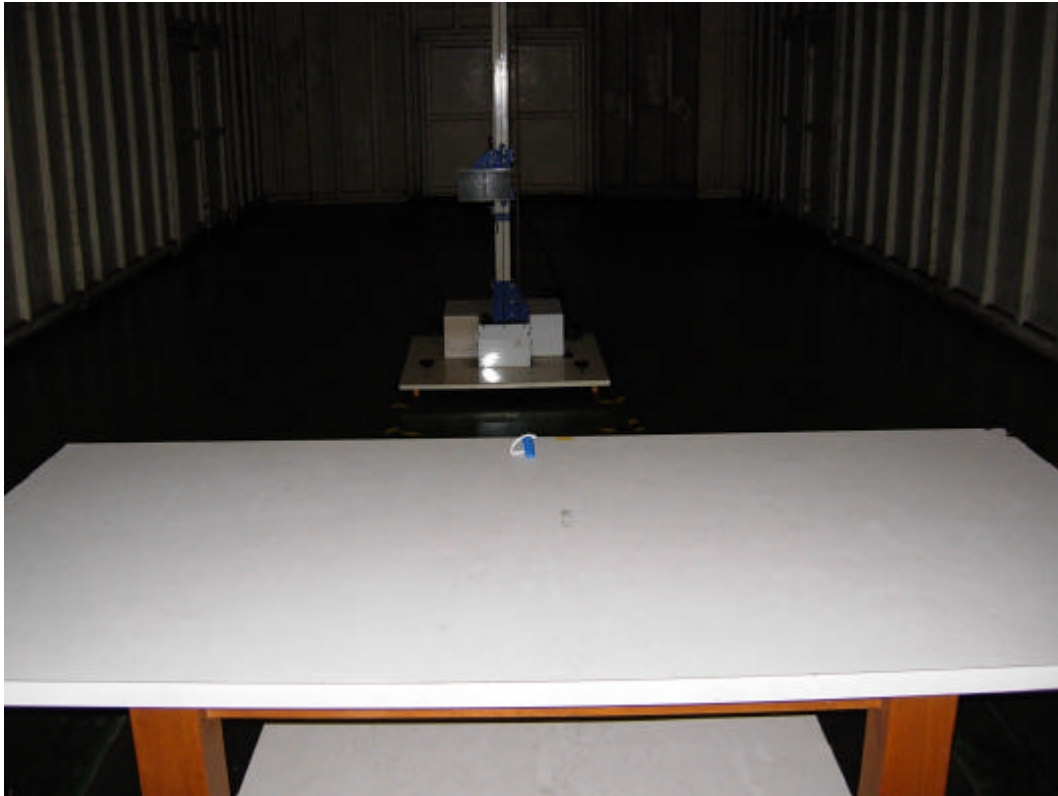
Back View of Radiated Test (Horn) Mode 1: Transmitter
