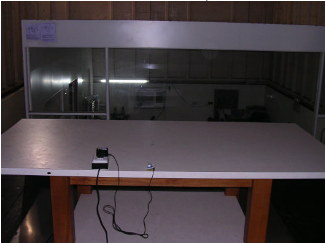
Back View of Radiated Test Mode 1: Transmitter (Charger)
