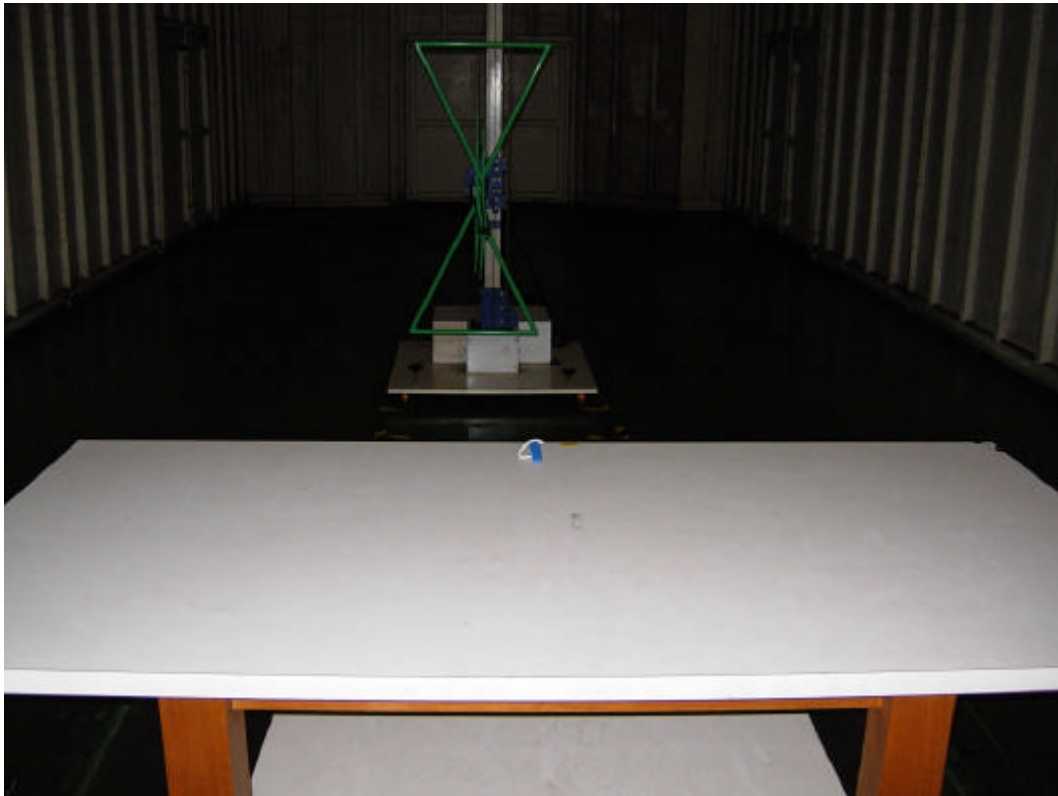
Front View of Radiated Test Mode 1: Transmitter
