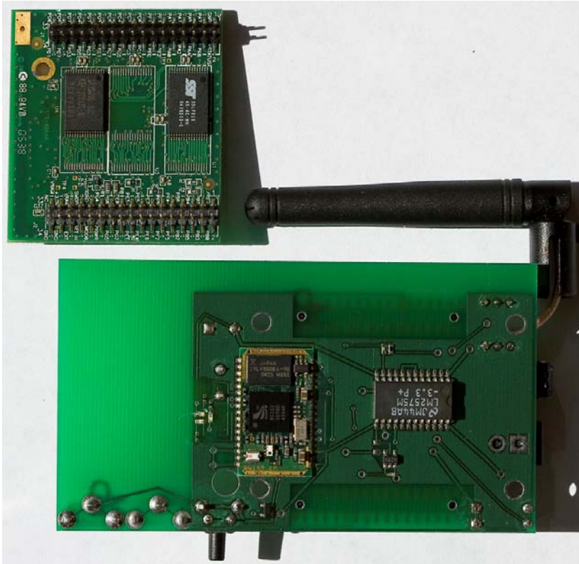
Yulock main board: top
