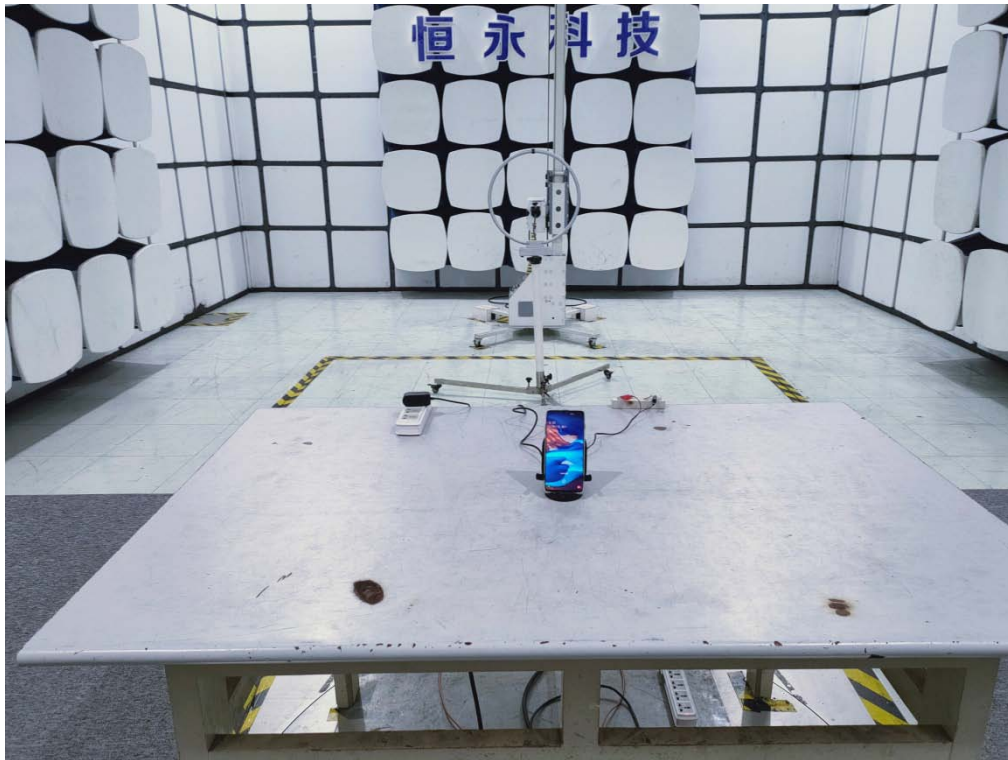
Radiated Test: 9K-30MHz
