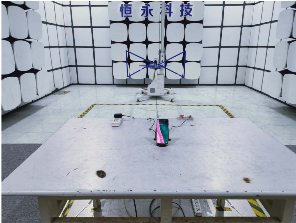
Radiated Test: 30M-1GHz
