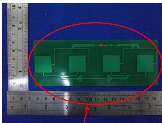
Original antenna
