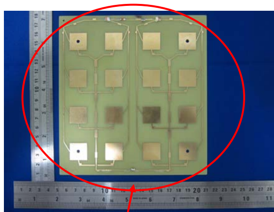
New antenna
