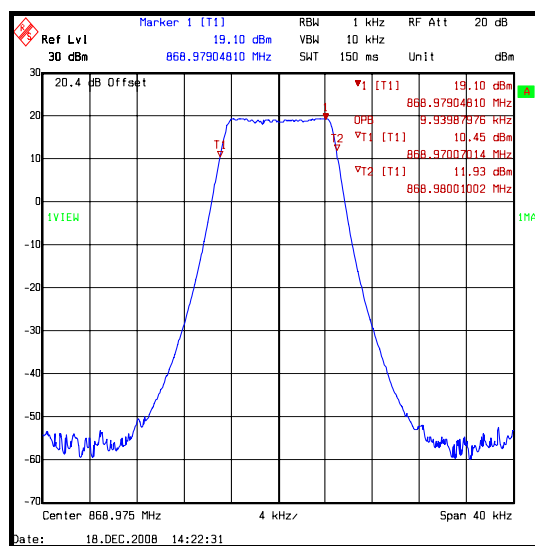
4-Level GFSK
