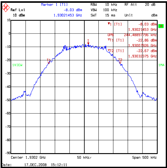
GMSK (GSM)
