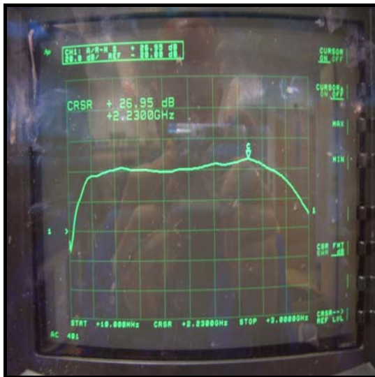
Gain flatness
