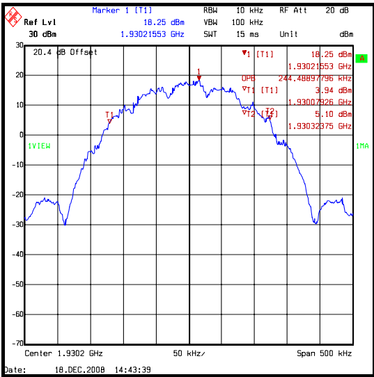
8PSK (EDGE)
