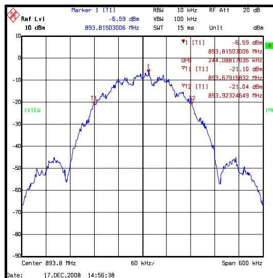
8PSK (EDGE)
