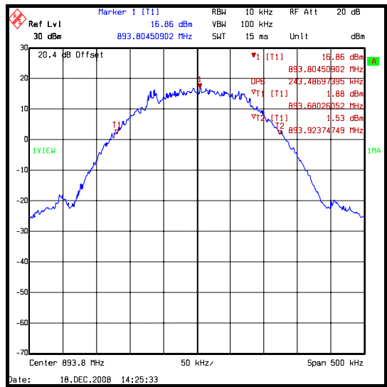
GMSK (GSM)
