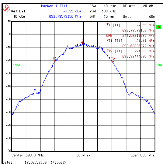
GMSK (GSM)
