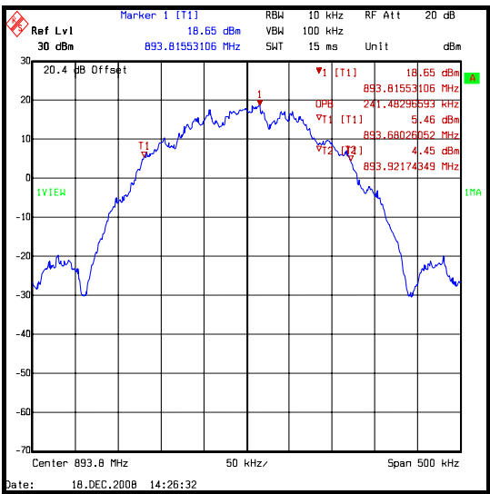
8PSK (EDGE)
