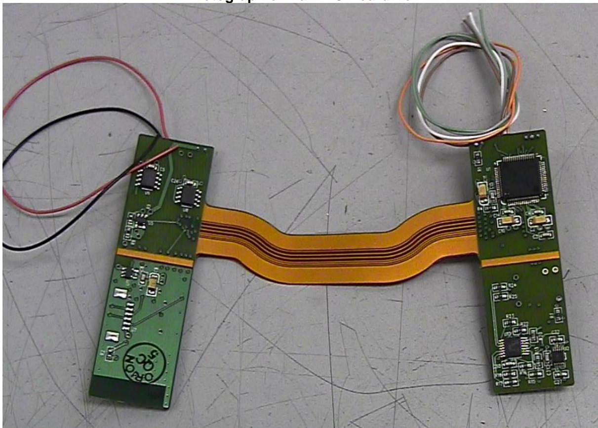
Photograph of Main PC Board-Foil
