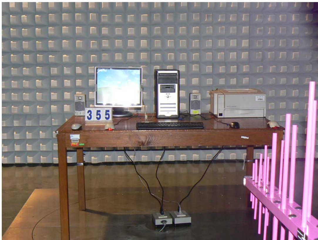
Radiated Disturbance
