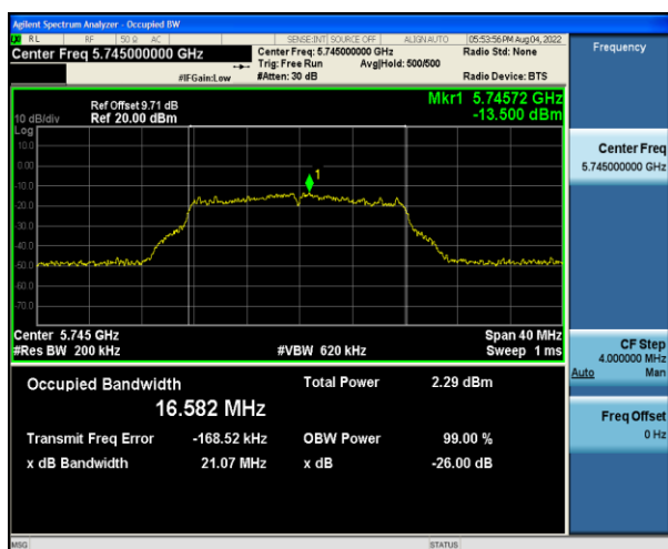
11a CH149
