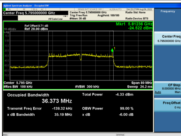
11ac(HT40) CH159
