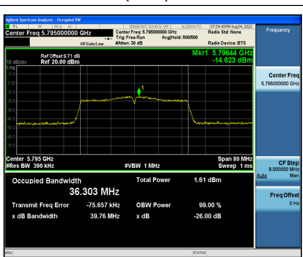
11ac(HT40) CH159
