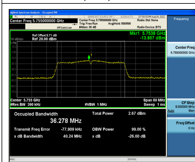
11ac(HT40) CH151
