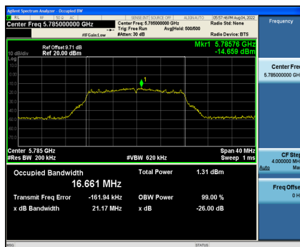
11a CH157
