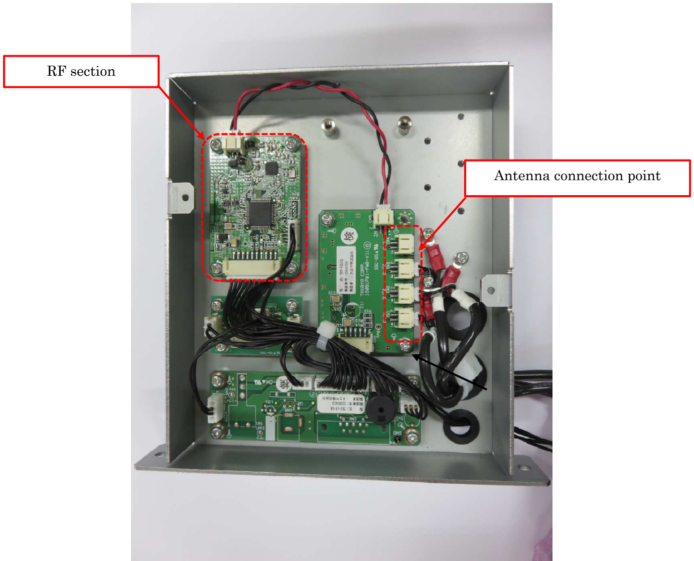
RF section and Antenna connection point (Surface)
