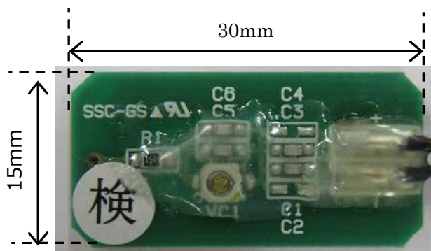
Front side of the Antenna
